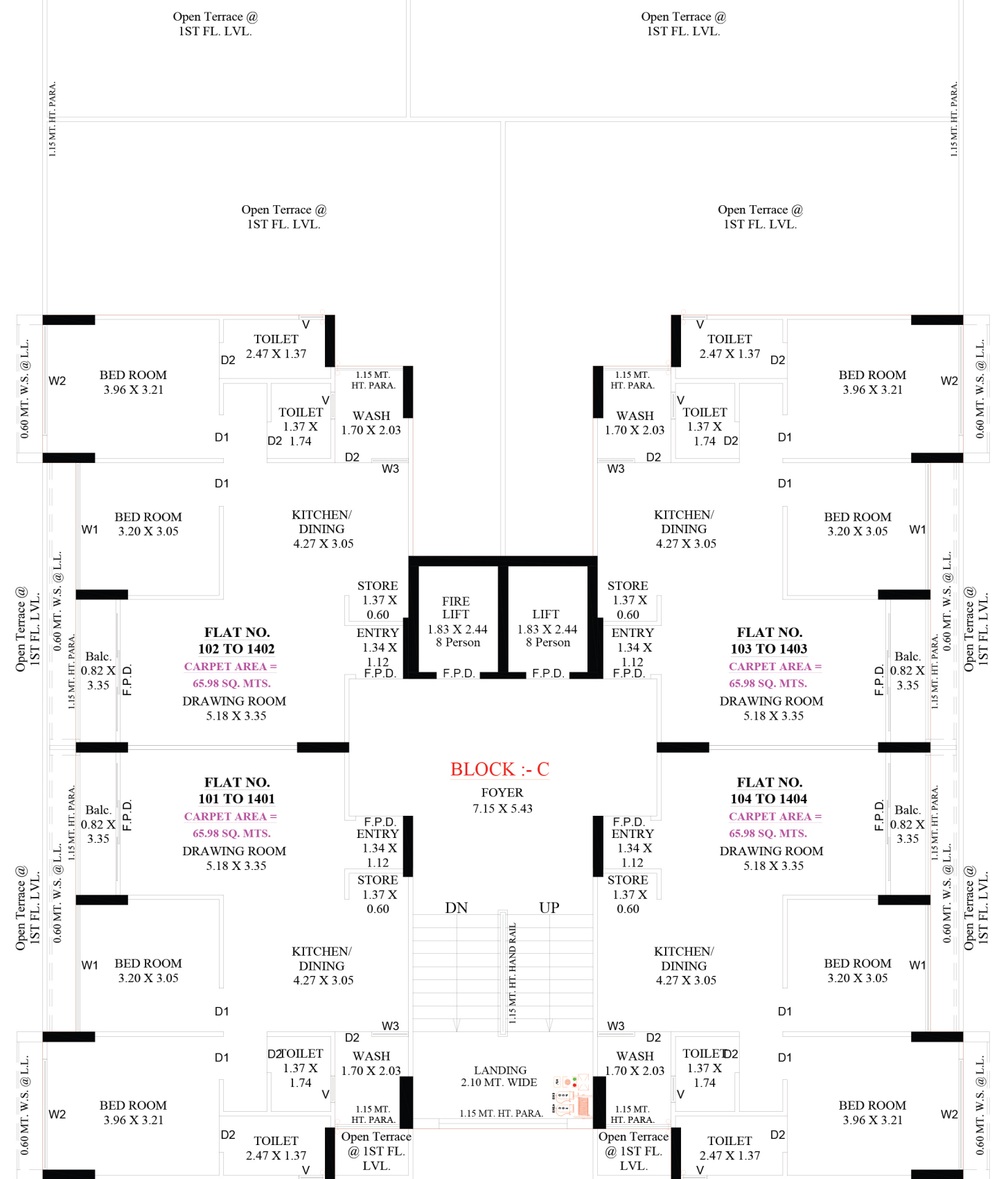
1 ST TO 4 TH , 6 TH , 7 TH , 9 TH TO 11 TH , 13 TH , 14 TH FLOOR PLAN NOTE :- ALL OUTER & INTERNAL WALL ARE OF 0.10 MT. TH. B/K WALL
