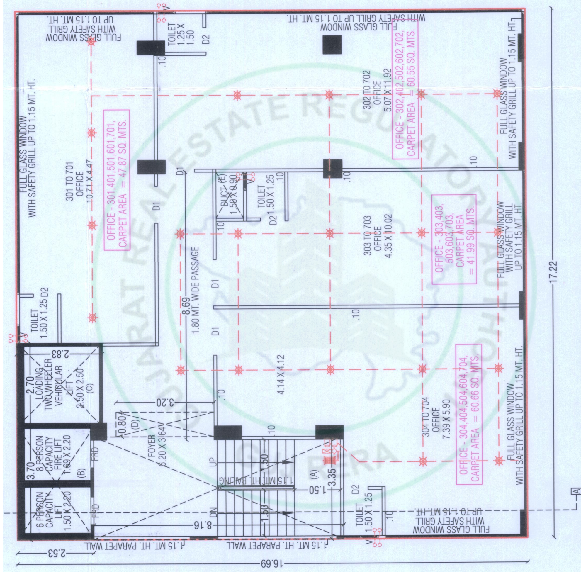
TYPICAL FLOOR PLAN ( 3RD TO 7TH FLOOR )
