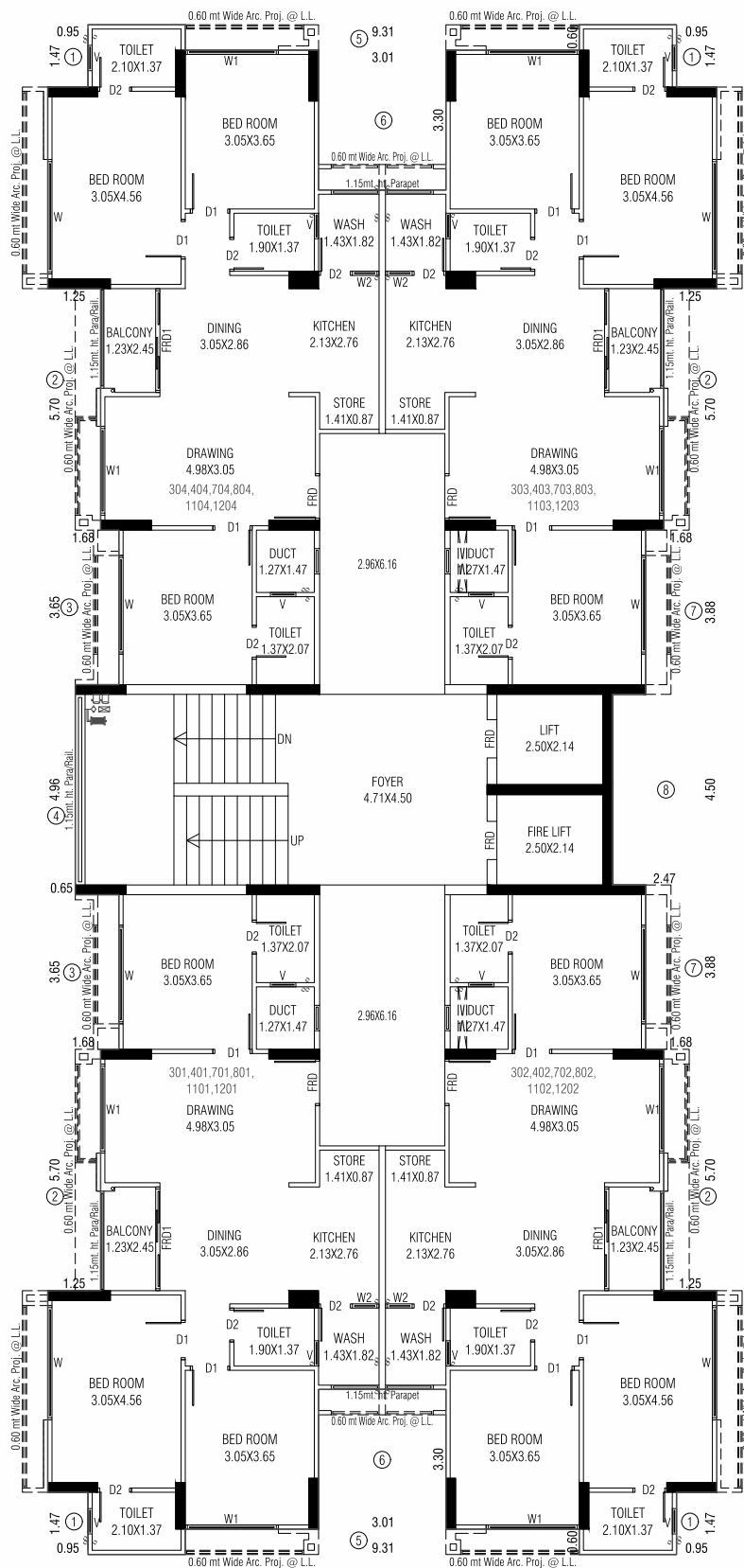
3RD,4TH,7TH,8TH,11TH & 12TH FLOOR PLAN
