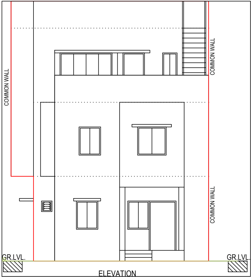
Elevation-3
