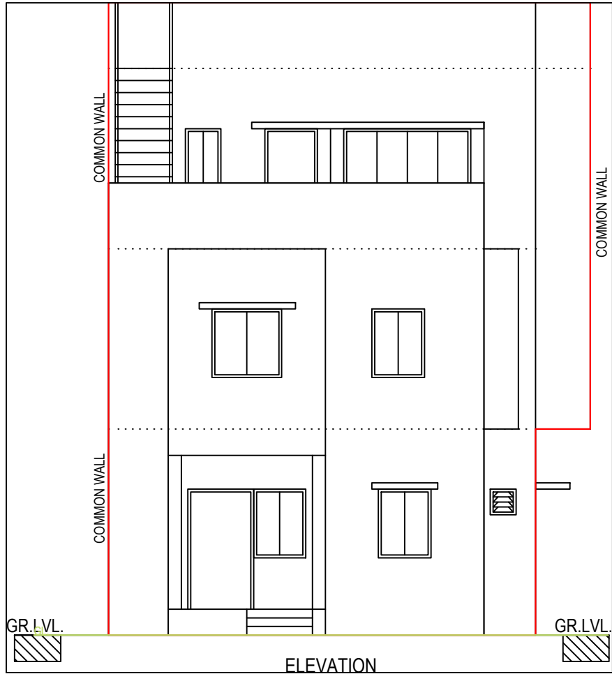
Elevation-2
