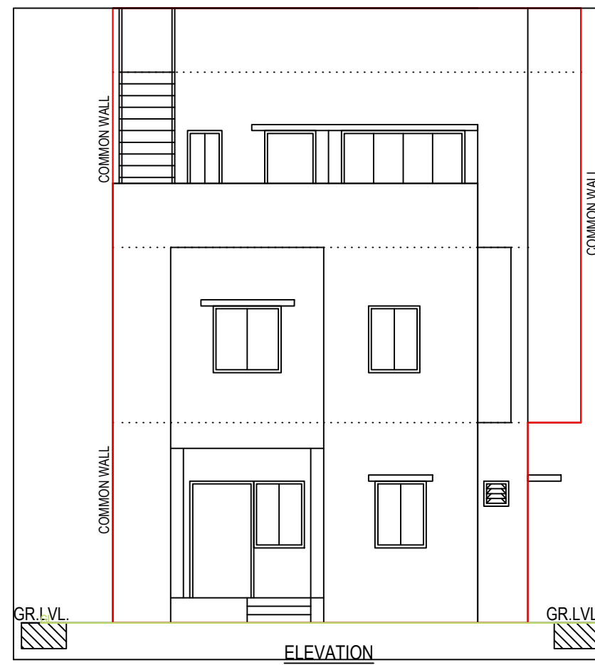
Elevation-10
