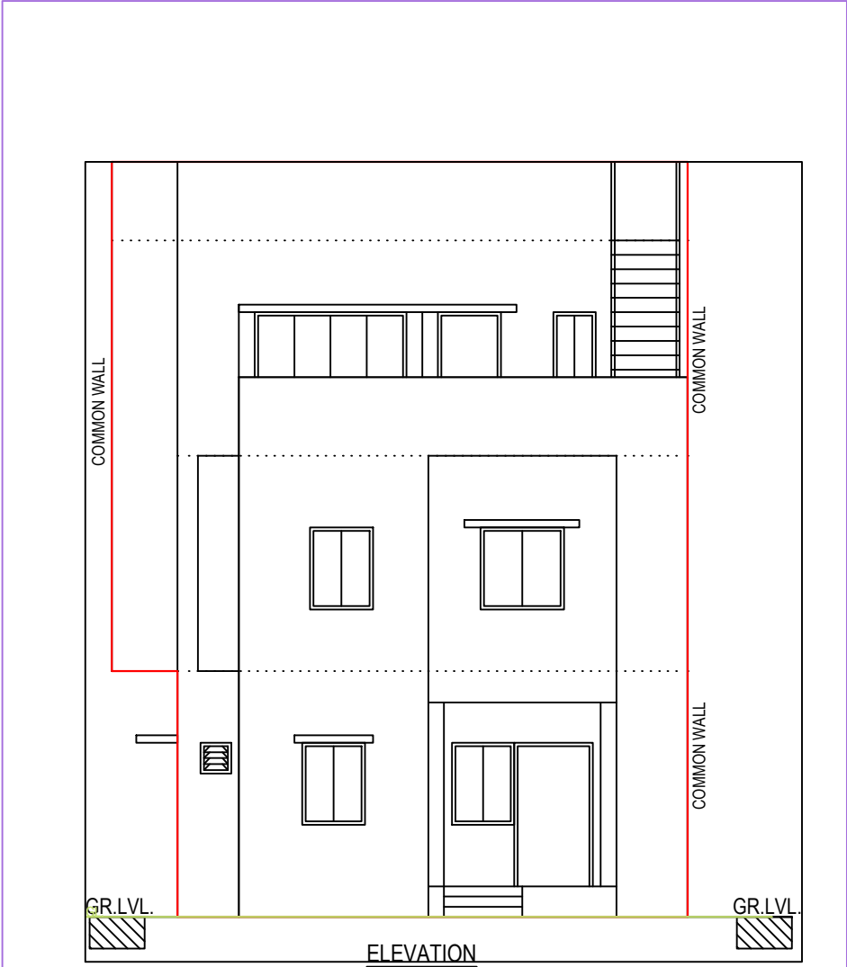
Elevation-12
