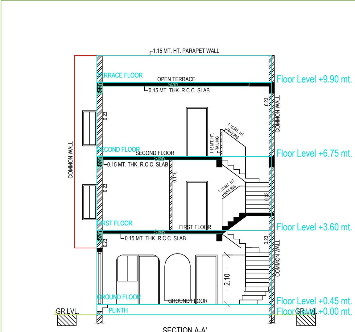
SECTION :- AA
