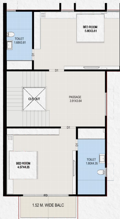
FIRST FLOOR PLAN ( UNIT NO:- 15, 17, 19 )
