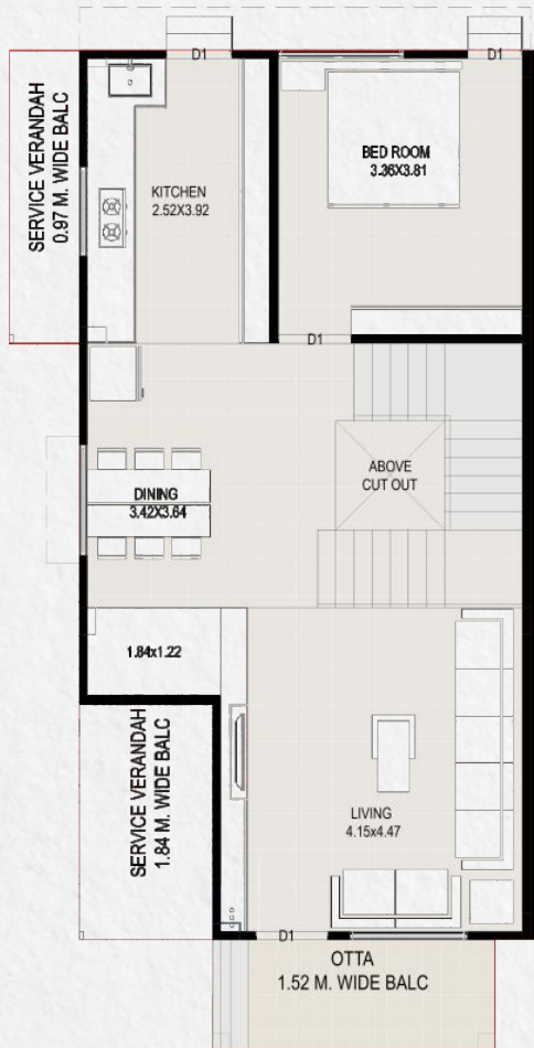
GROUND FLOOR PLAN ( UNIT NO:- 22, 26)
