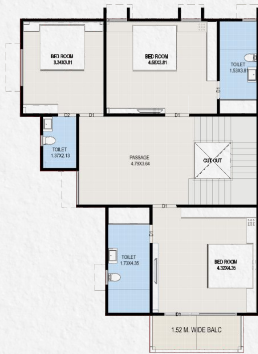
FIRST FLOOR PLAN( UNIT NO:- 36 )
