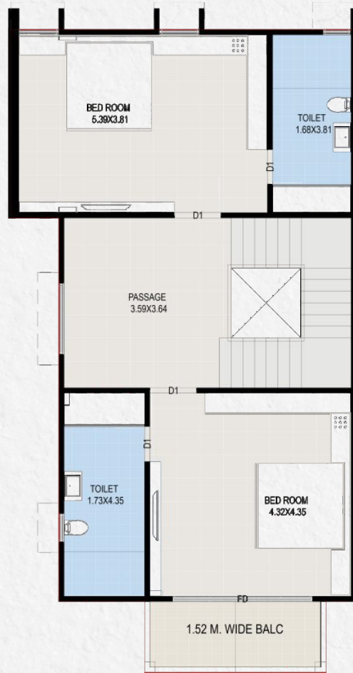
FIRST FLOOR PLAN( UNIT NO:- 35 )
