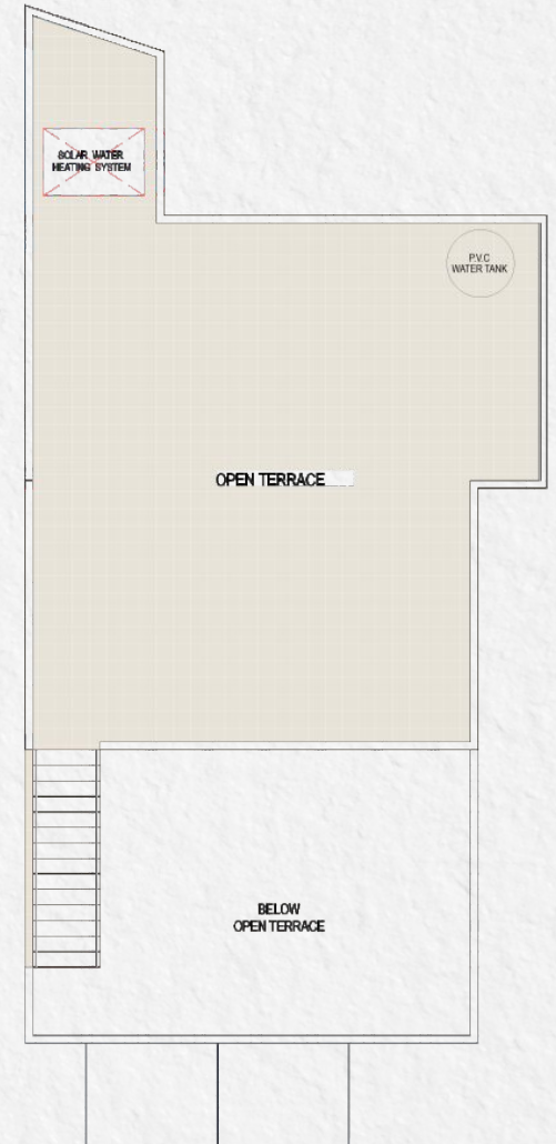
TERRACE FLOOR PLAN ( UNIT NO:- 30 )
