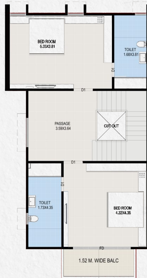
FIRST FLOOR PLAN (UNIT NO:- 02, 04, 06, 08, 10, 33)
