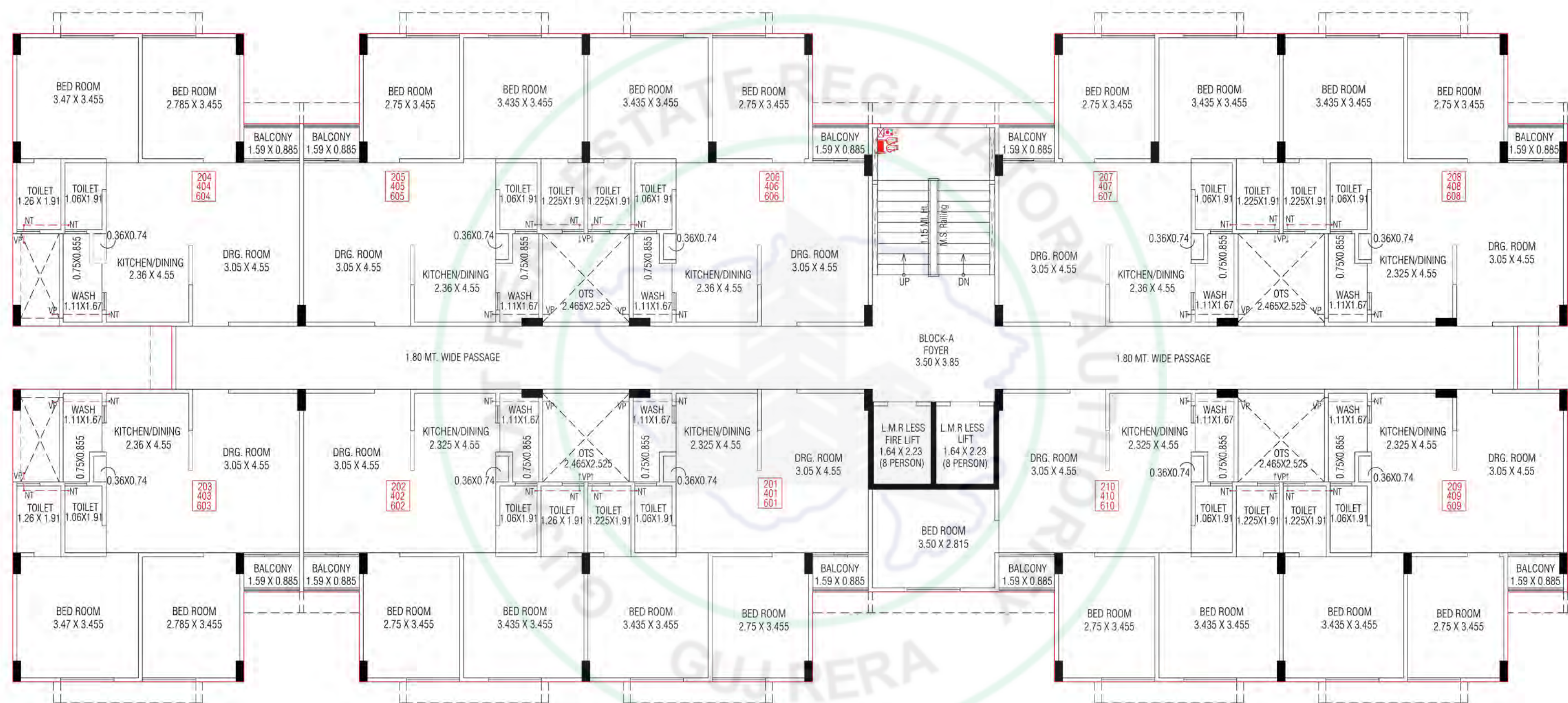
2nd, 4th. & 6th. FLOOR PLAN
