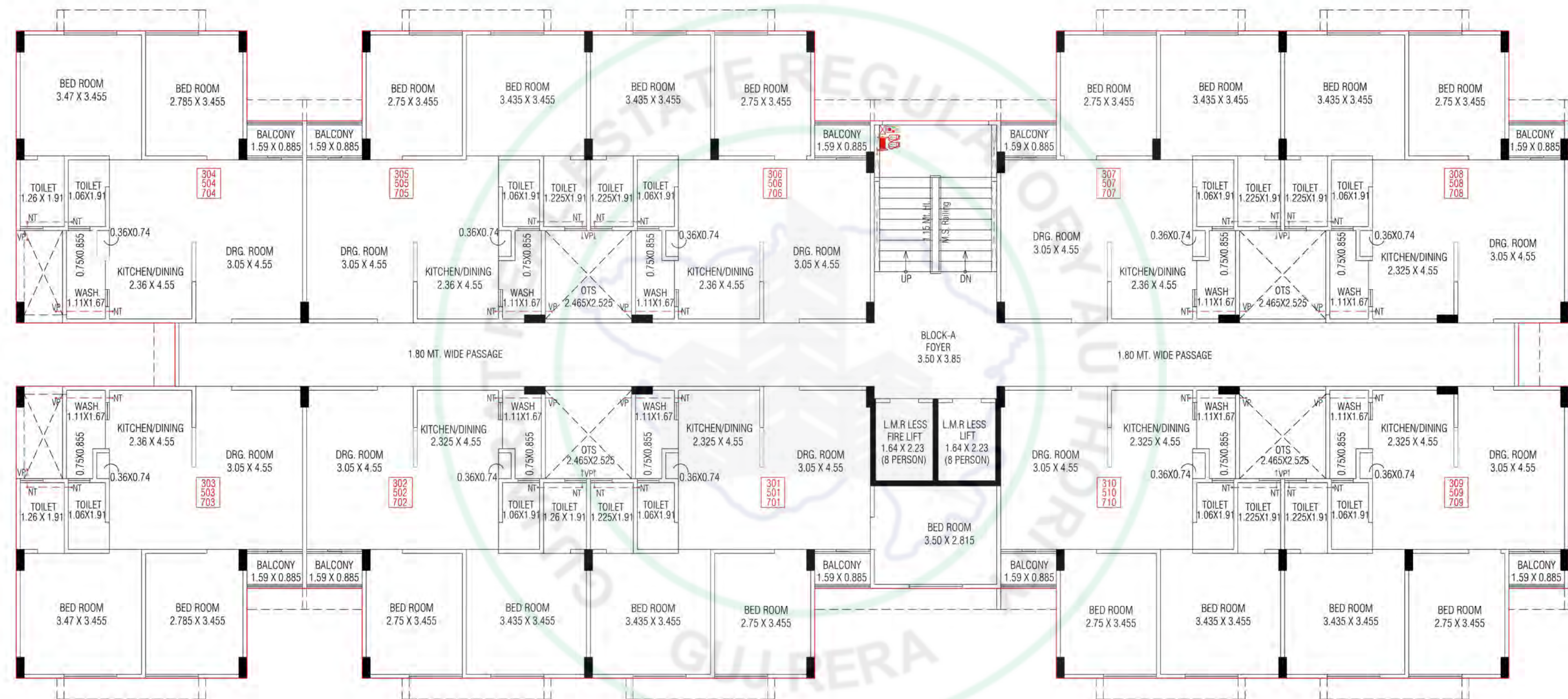
3rd.,5th. & 7th. FLOOR PLAN
