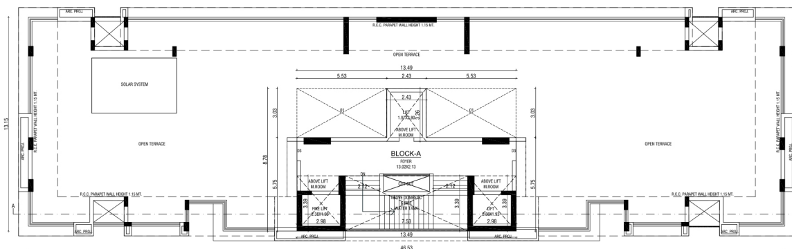
TERRACE PLAN
