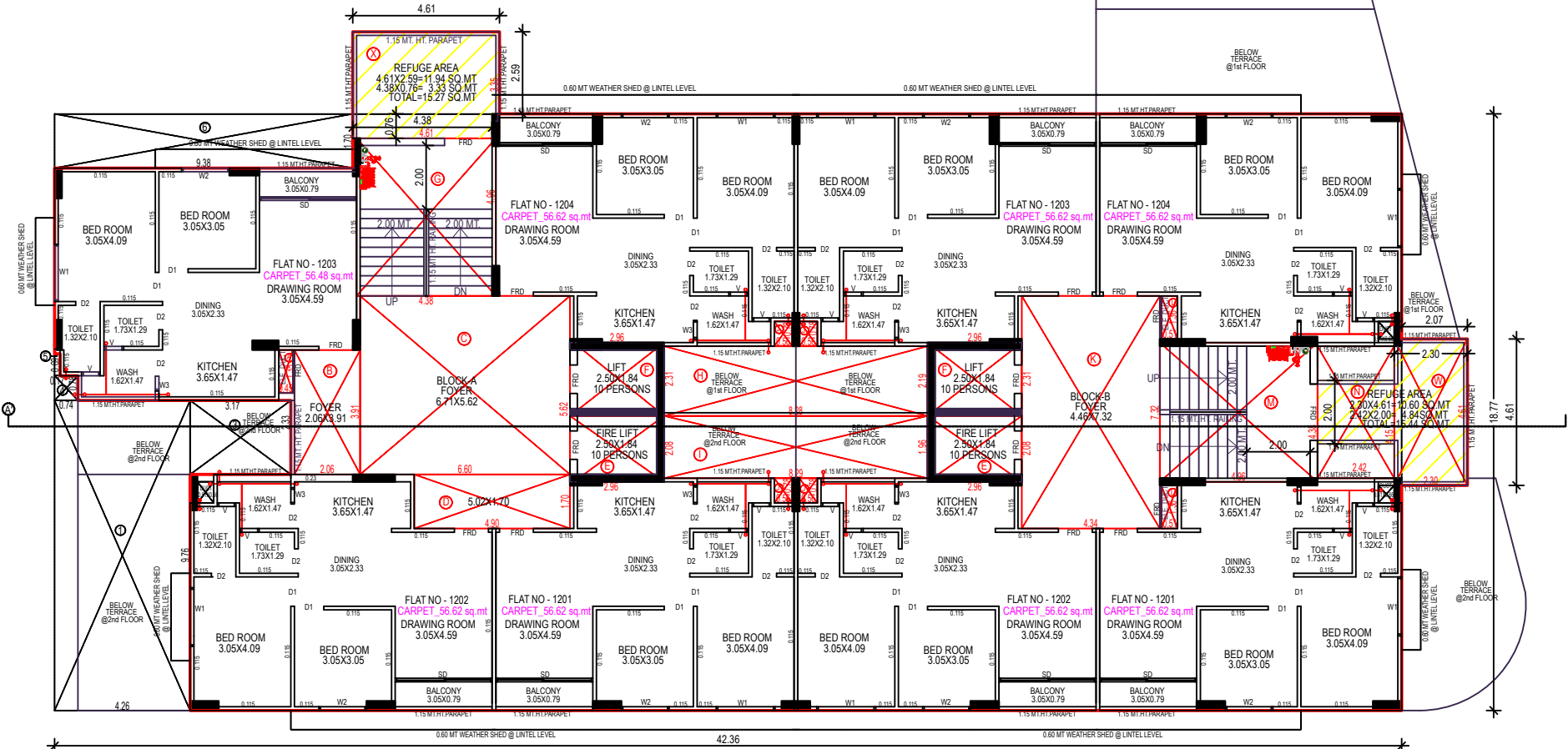
12th FLOOR PLAN
