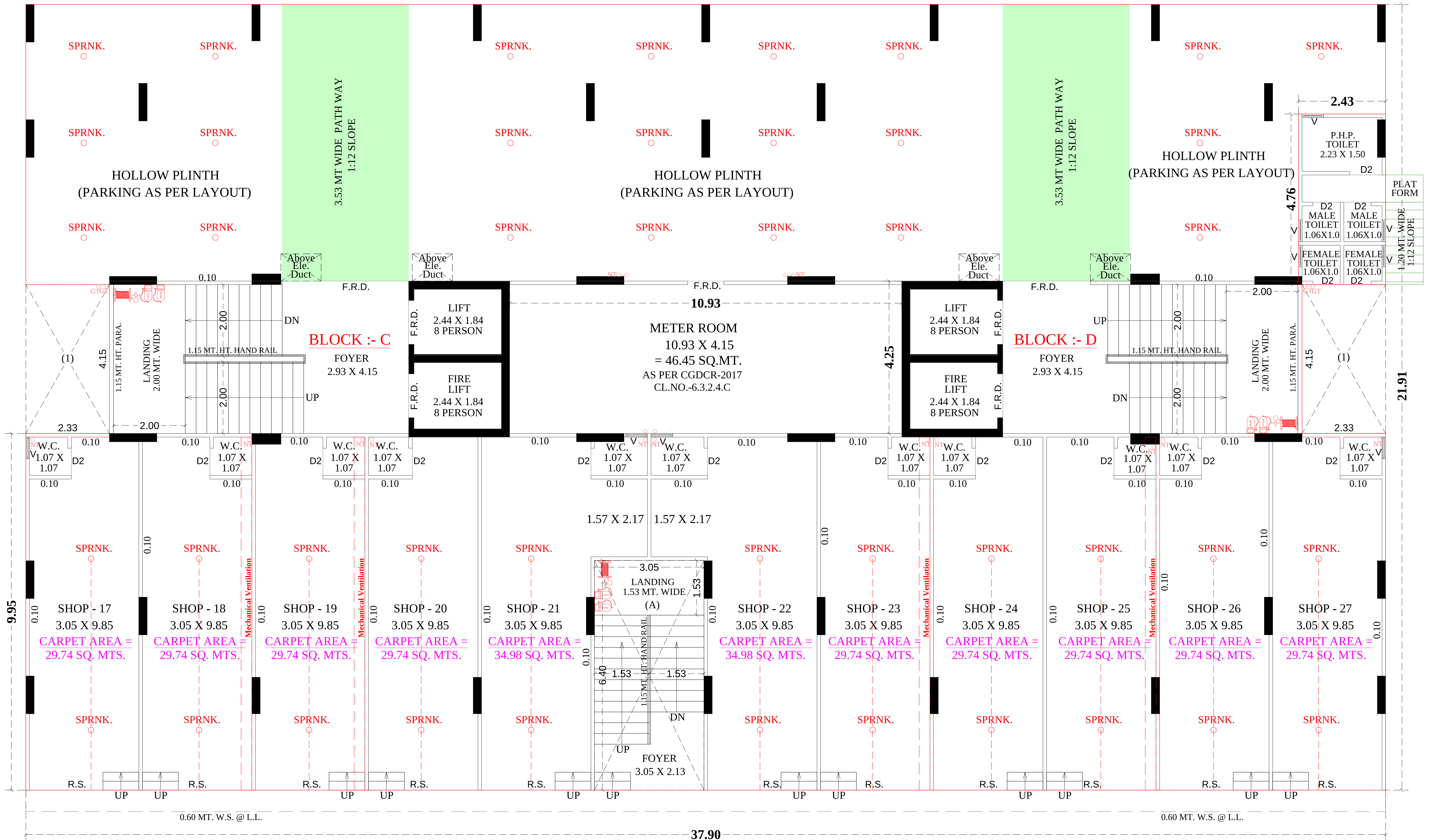
GROUND FLOOR PLAN (HOLLOW PLINTH+SOLID PLINTH)
