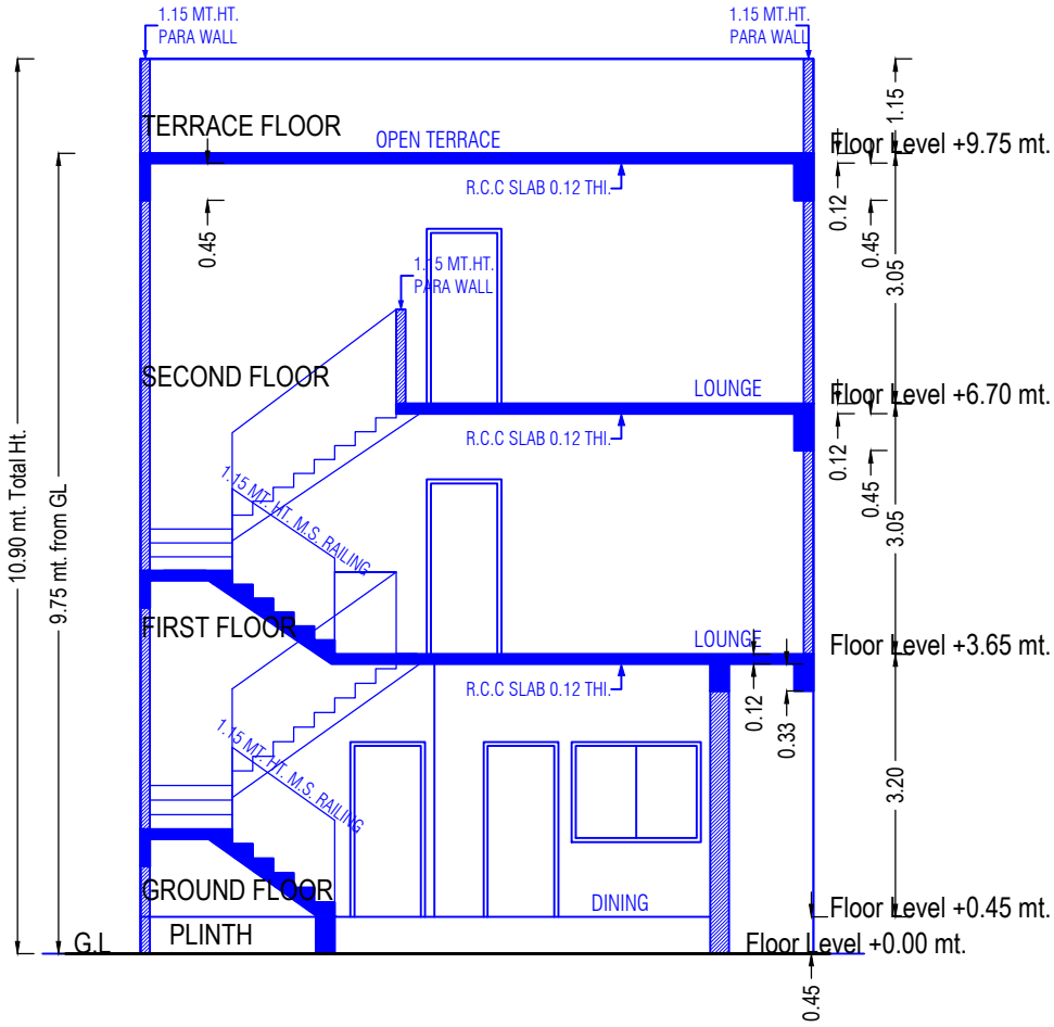
SECTION
