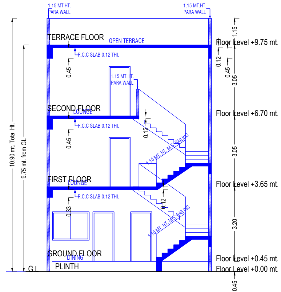
SECTION
