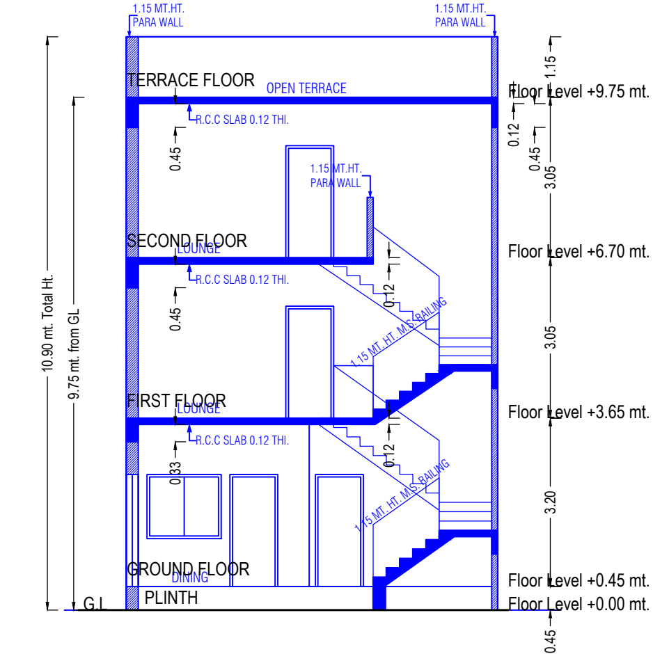
SECTION
