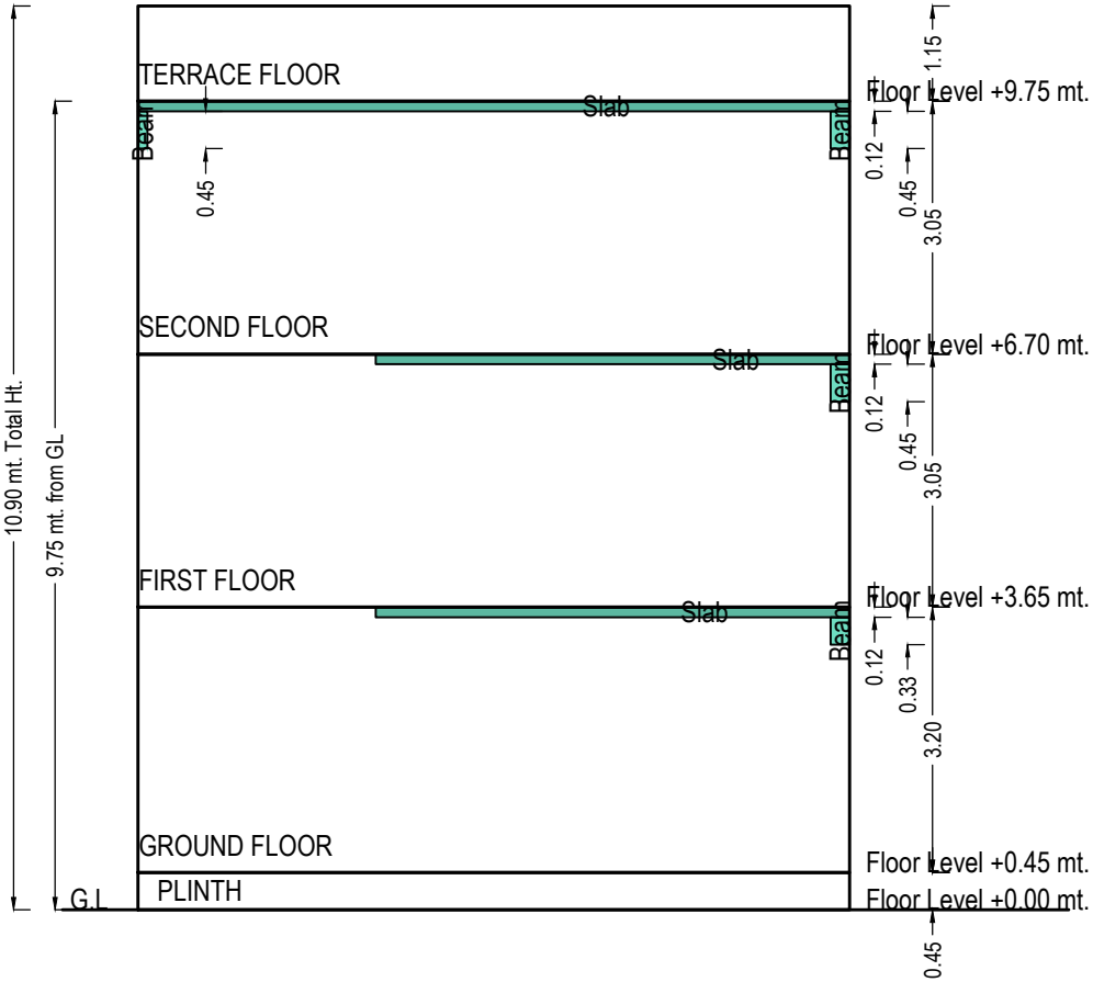
SECTION
