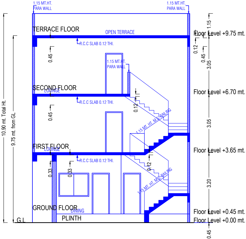
SECTION
