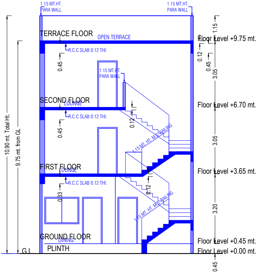
SECTION
