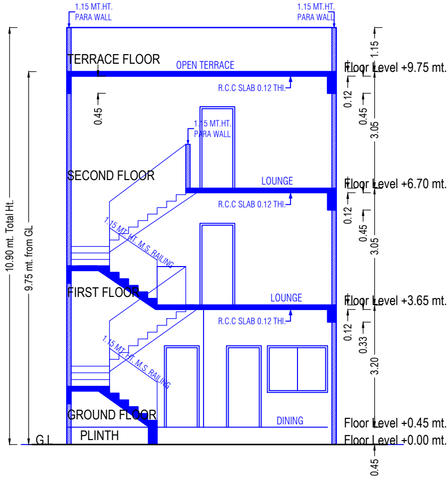
SECTION
