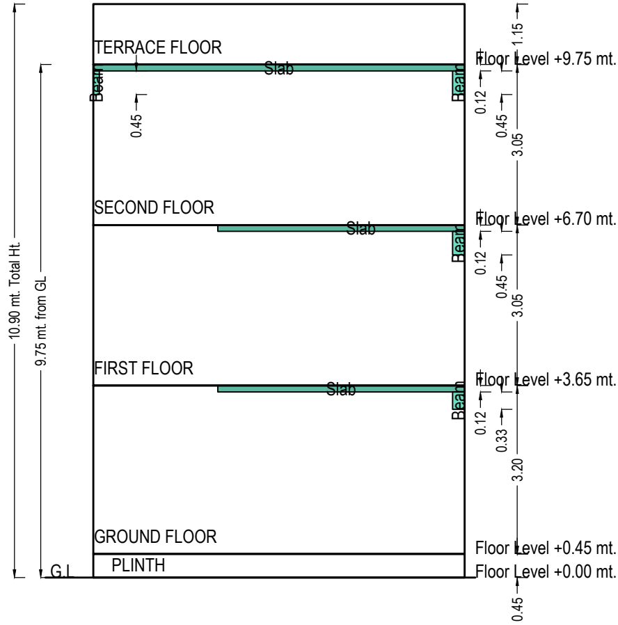
SECTION
