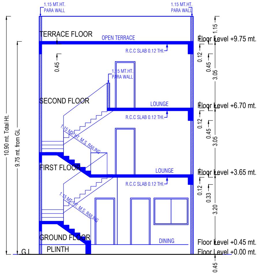
SECTION
