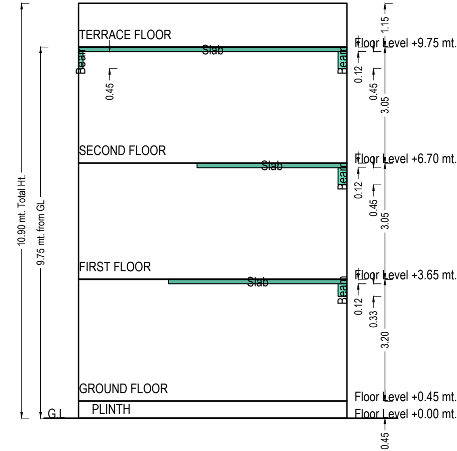
SECTION
