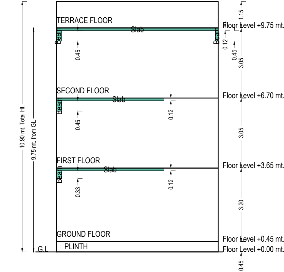
SECTION
