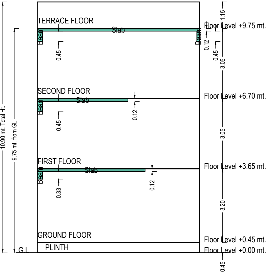
Sectional Diagram
