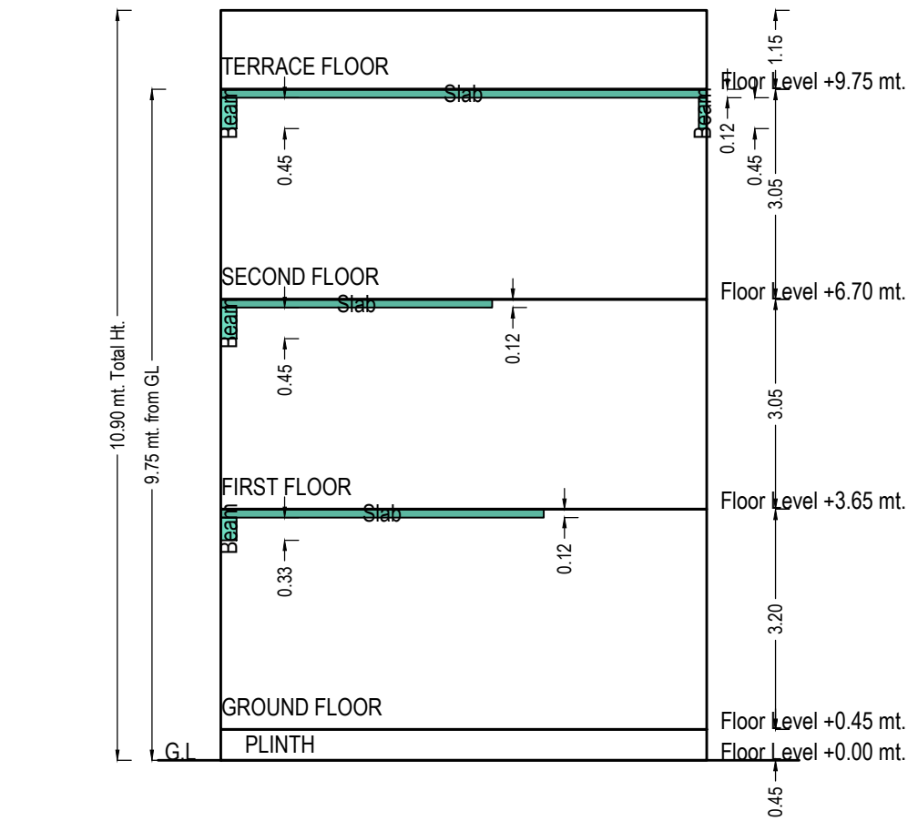
SECTION
