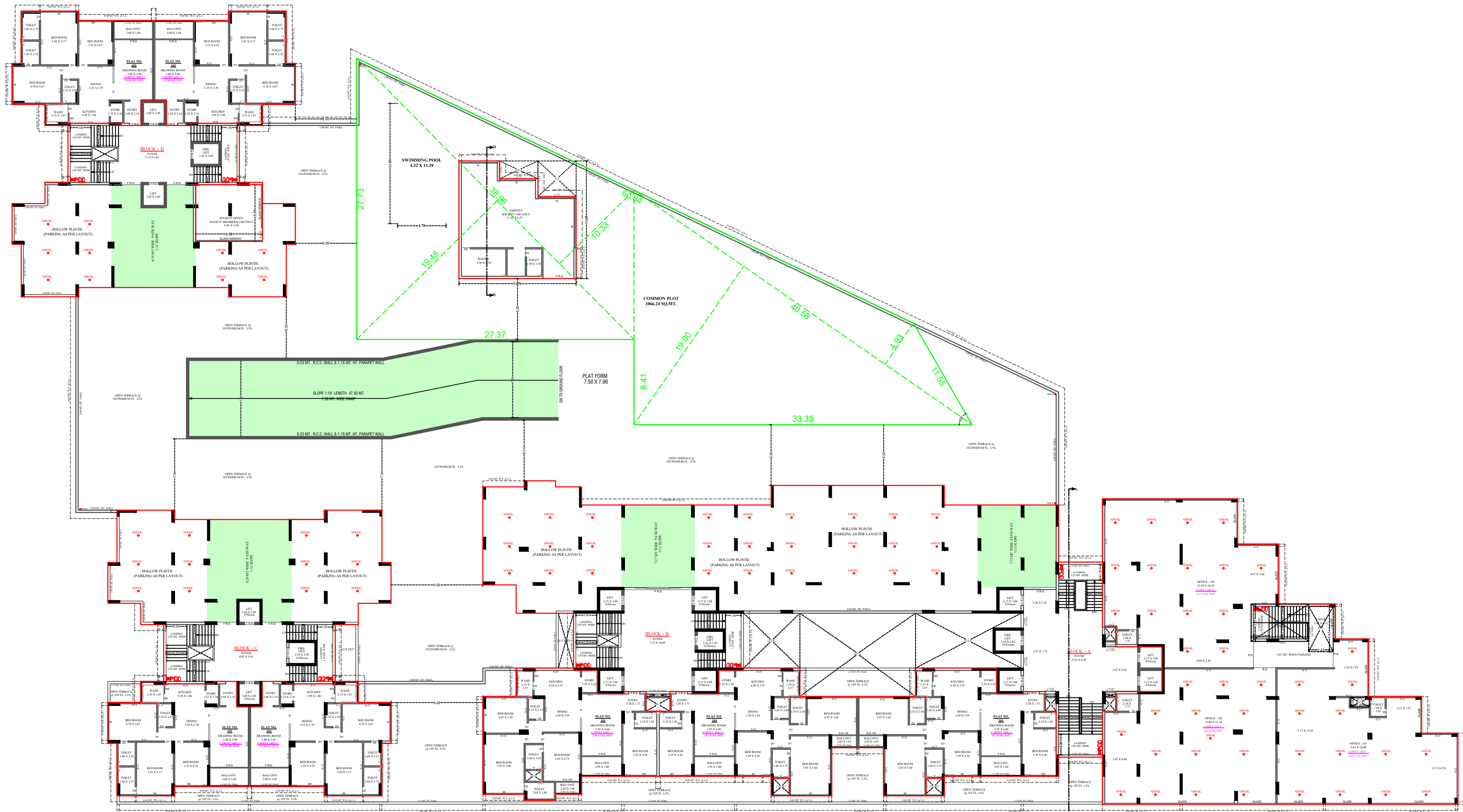
1ST / PODIUM FLOOR PLAN
