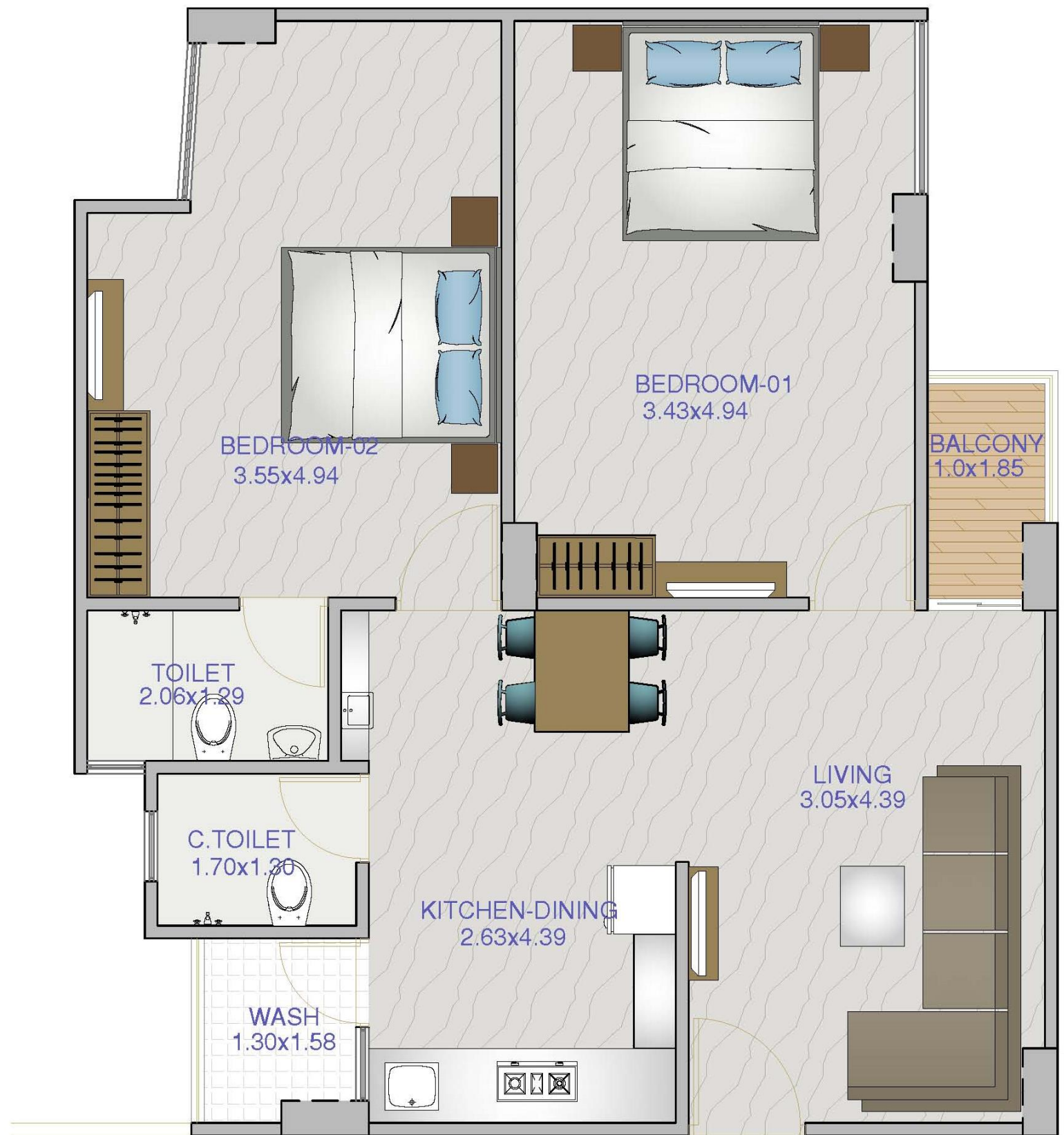
Typical Unit Plan
