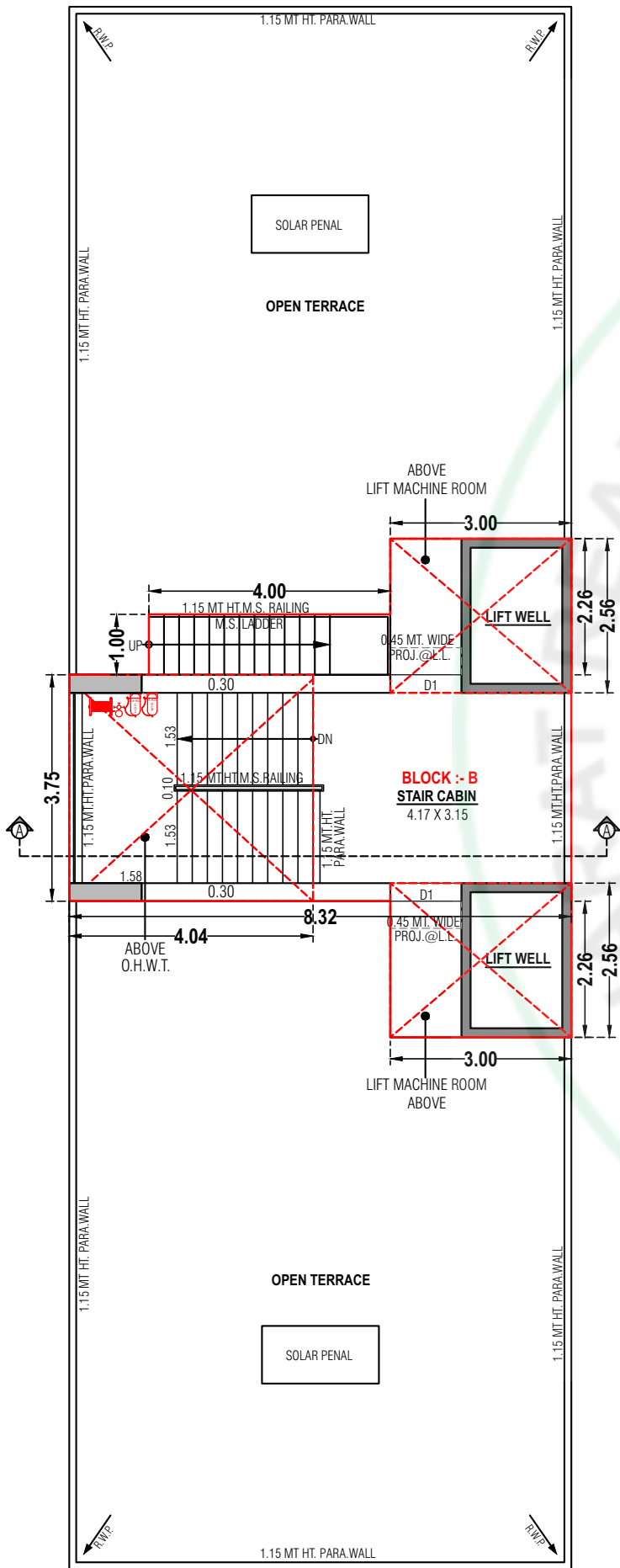
OPEN TERRACE PLAN WITH STAIR CABIN, LIFT MACHINE RM, O.H.W.T., PLAN
