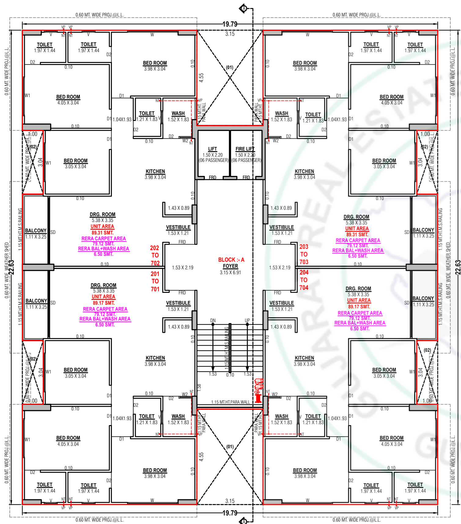
2ND. TO 7TH. FLOOR PLAN
