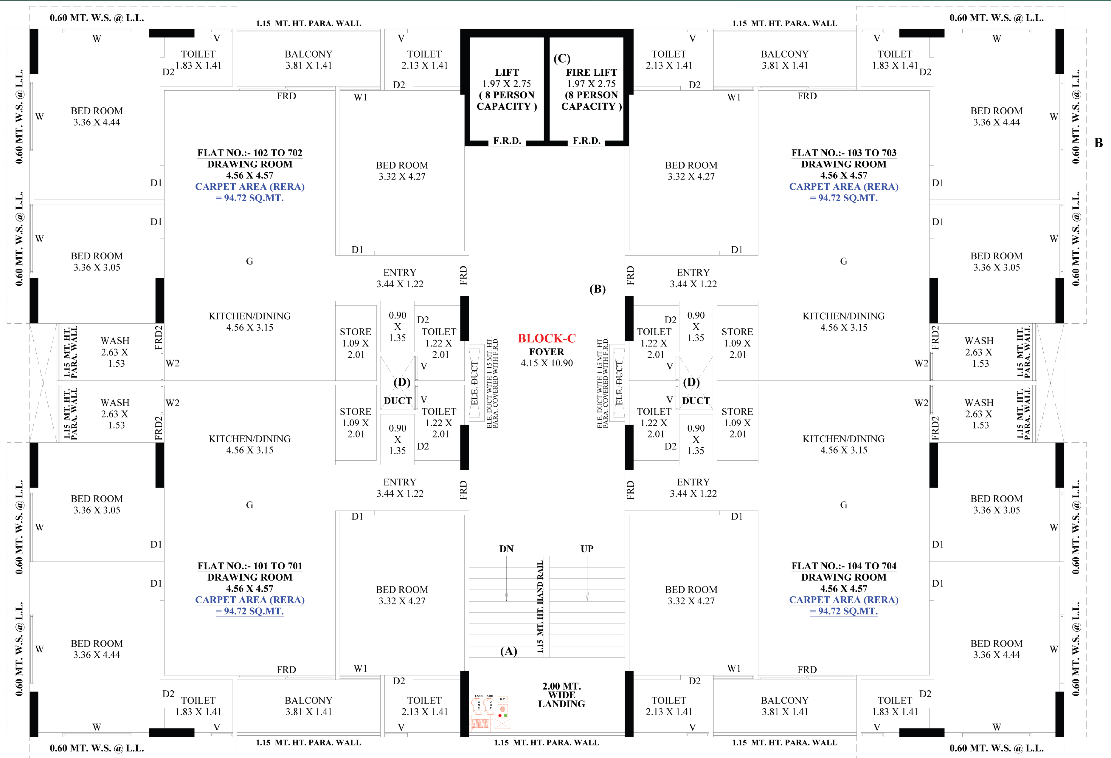
TYPICAL FLOOR LAYOUT plan BLOCK - C
