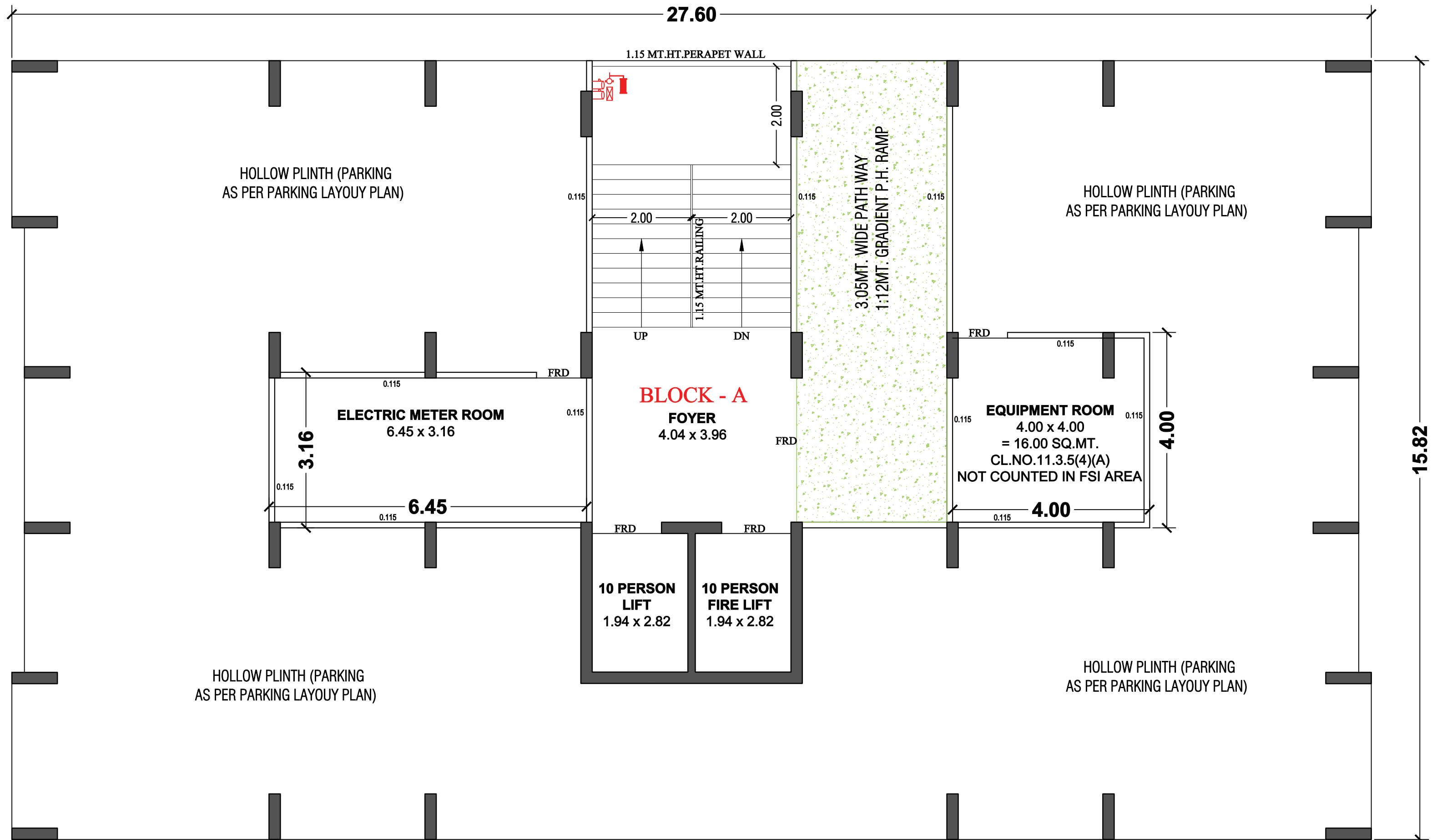
GROUND FLOOR PLAN ( HOLLOW PLINTH )
