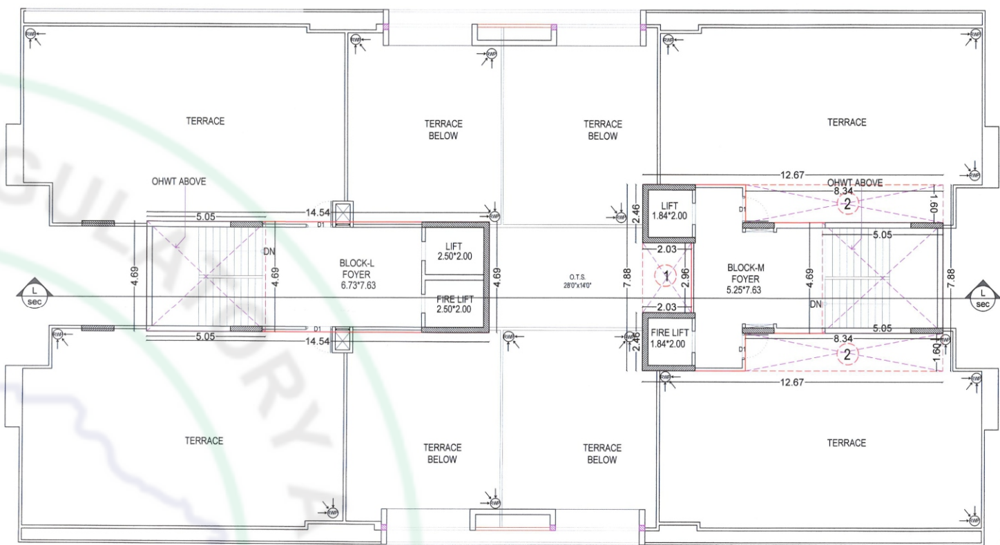
TERRACE FLOOR PLAN BLOCK L+M
