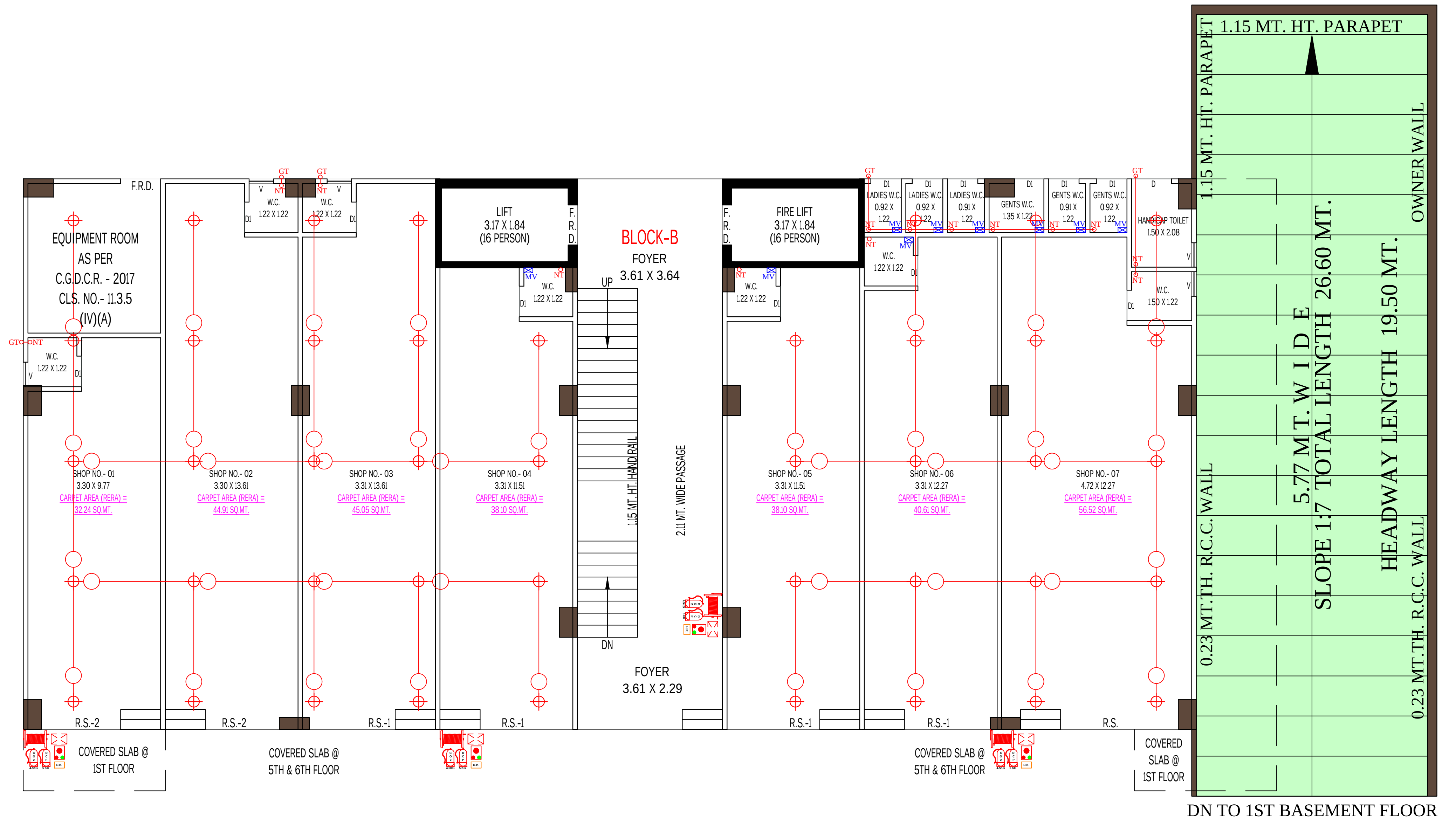
GROUND FLOOR PLAN BLOCK - B
