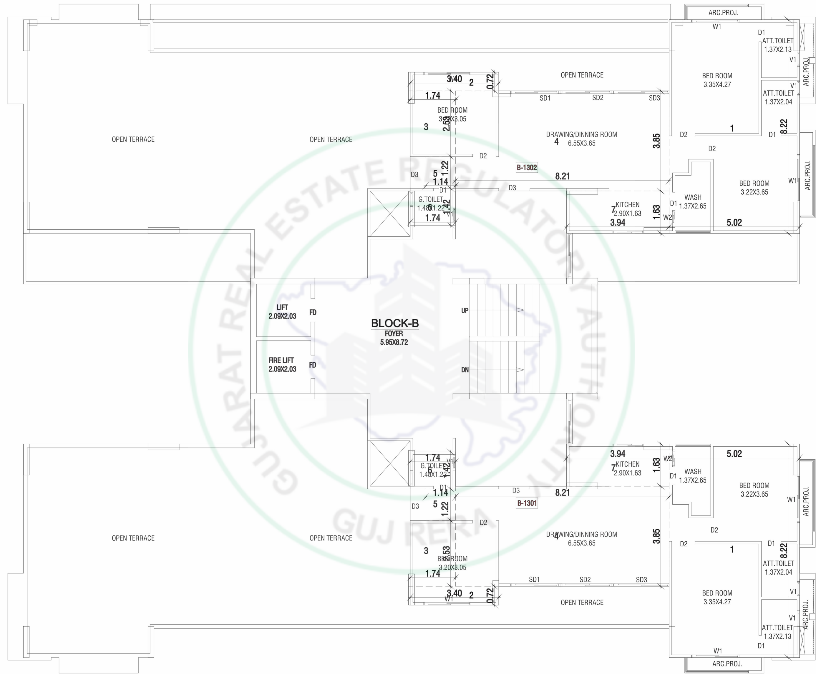
UNIT BUILTUP AREA CALCULATION FOR 13TH FLOOR (BLOCK B)
