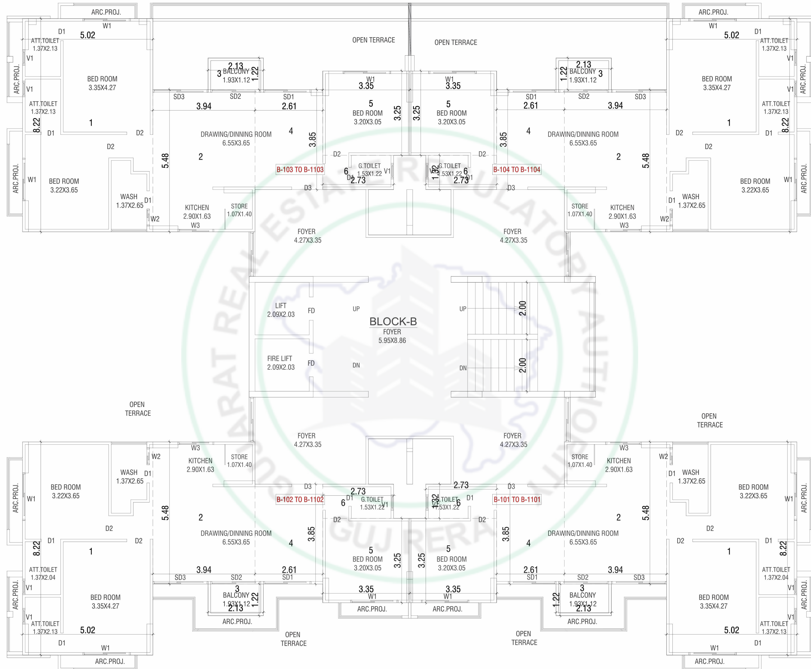
UNIT BUILTUP AREA CALCULATION FOR TYP. FLOOR (BLOCK B)(1ST TO 12TH FLOOR)
