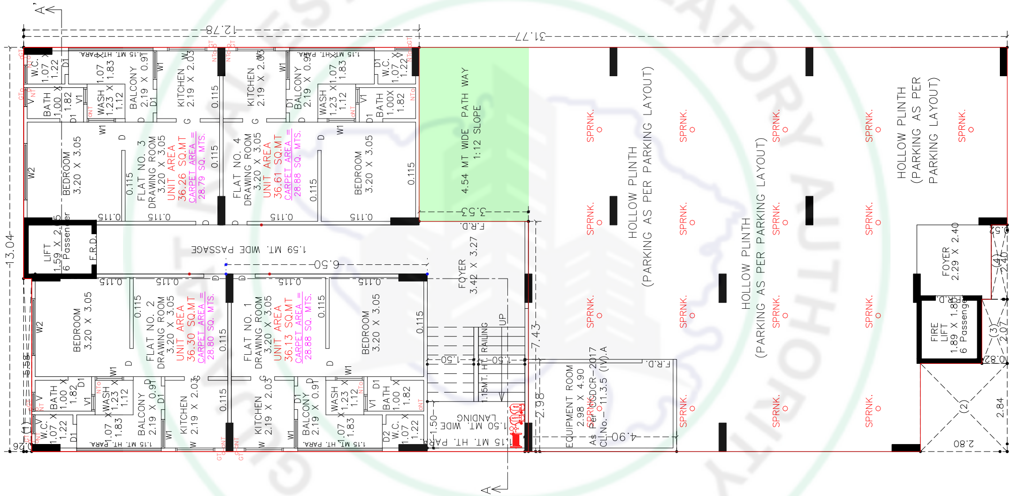
GROUND FLOOR PLAN (HOLLOW PLINTH+SOLID PLINTH)
