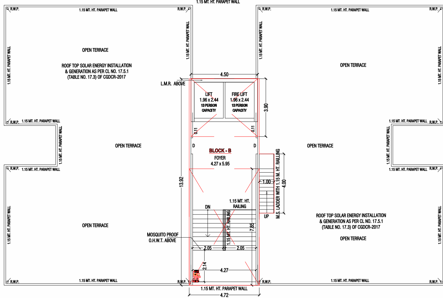
OPEN TERRACE WITH STAIR CABIN, L.M.R. & O.H.W.T. PLAN
