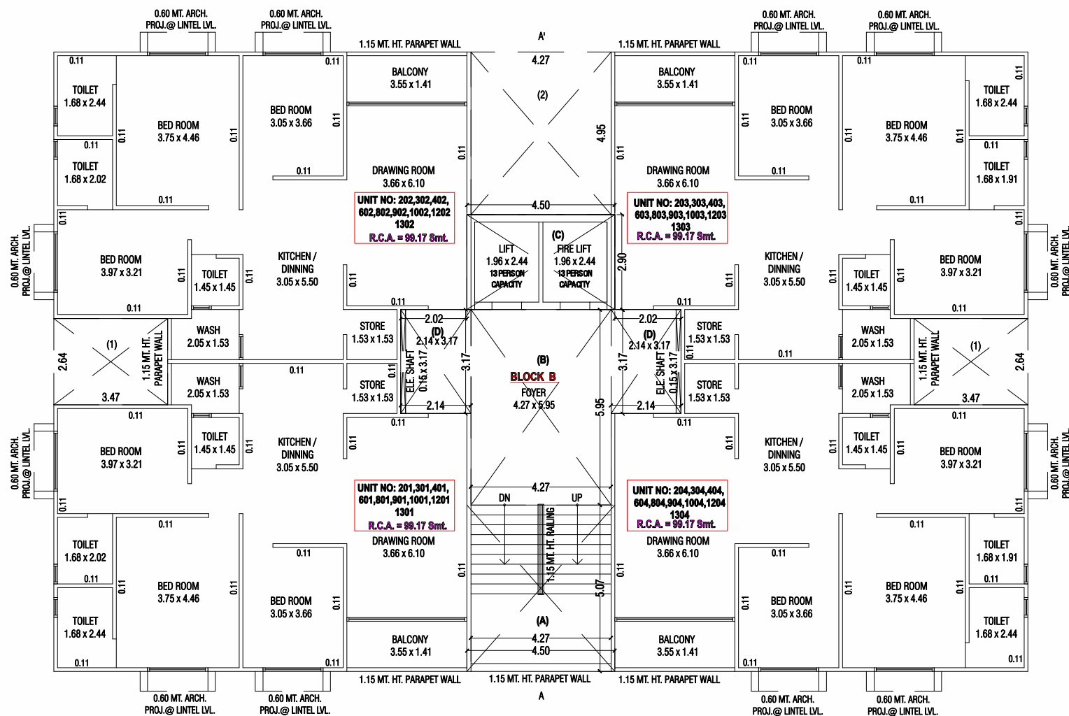
2nd to 4th, 6th, 8th to 10th, 12th & 13th FLOOR PLAN
