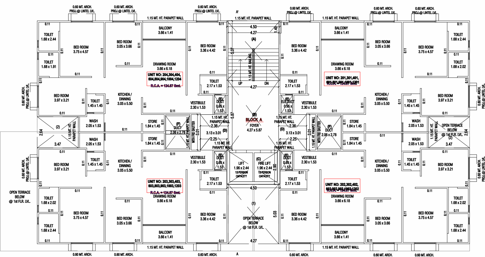
2nd to 4th, 6th, 8th to 10th & 12th FLOOR PLAN
