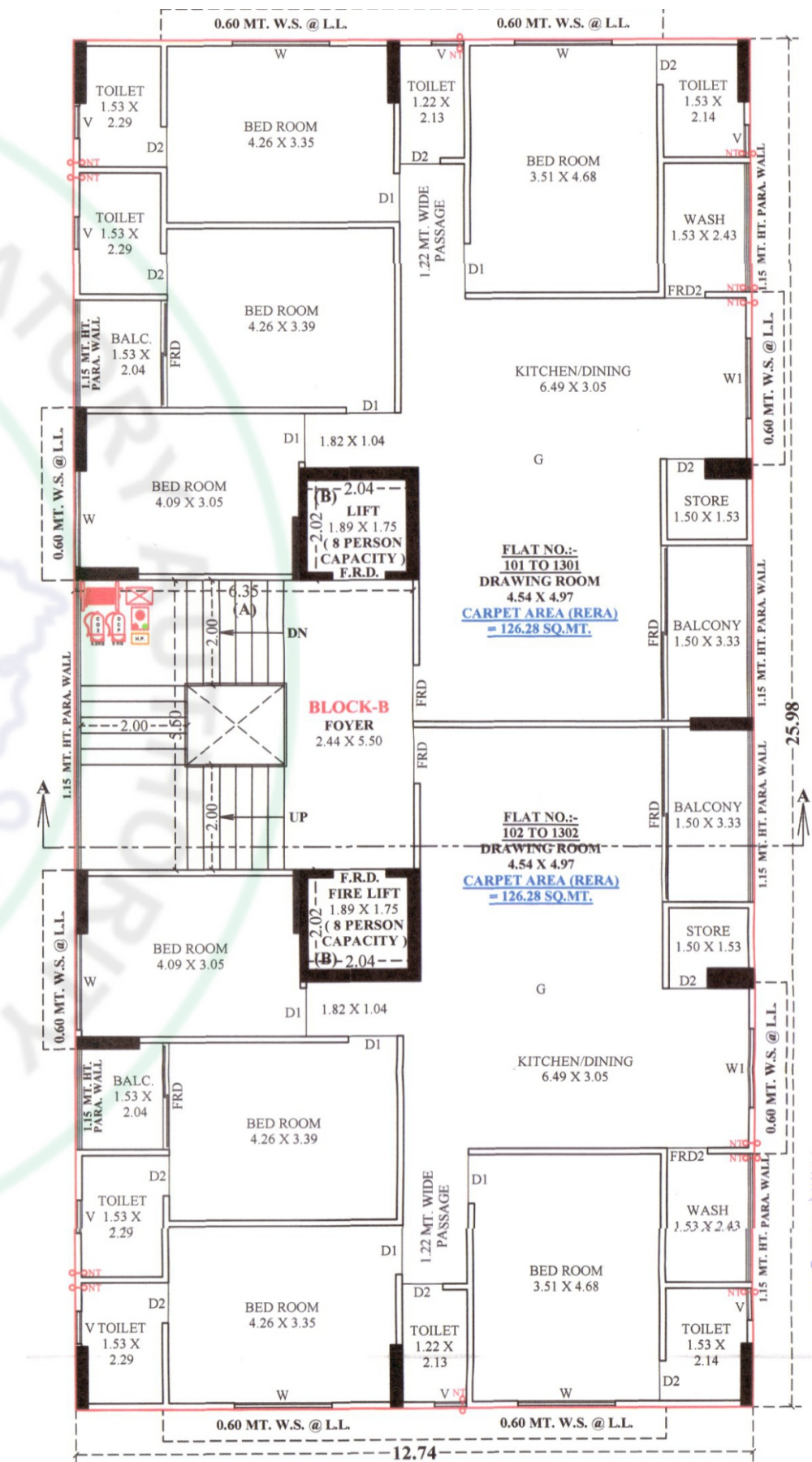
TYPICAL ( 1ST TO 13TH ) FLOOR PLAN NOTE :- ALL OUTER & INTERNAL WALL ARE OF 0.115 MT. TH. B/K WALL
