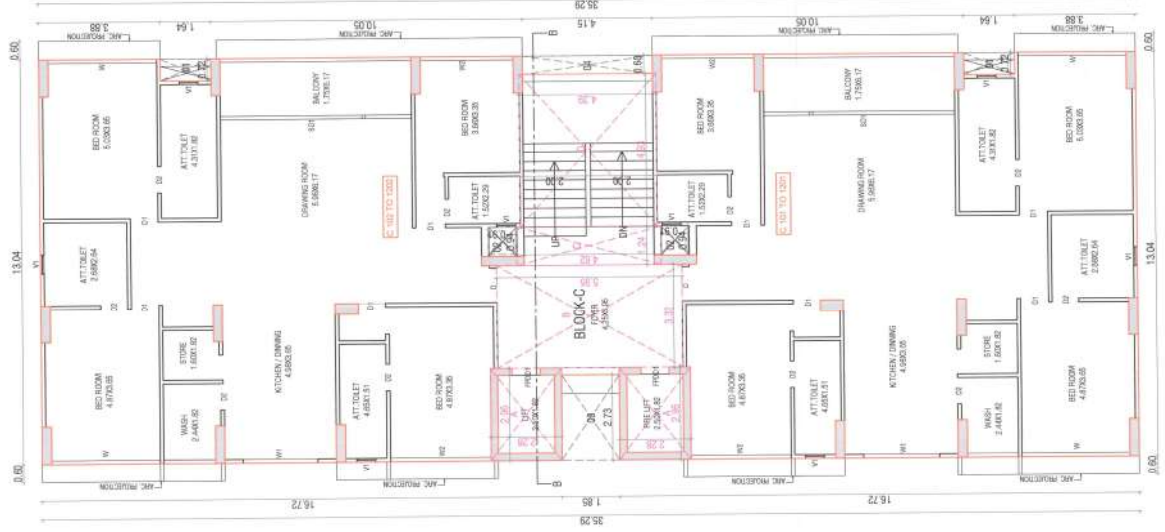
TYPICAL FLOOR PLAN (1st. FLOOR TO 12th. FLOOR)
