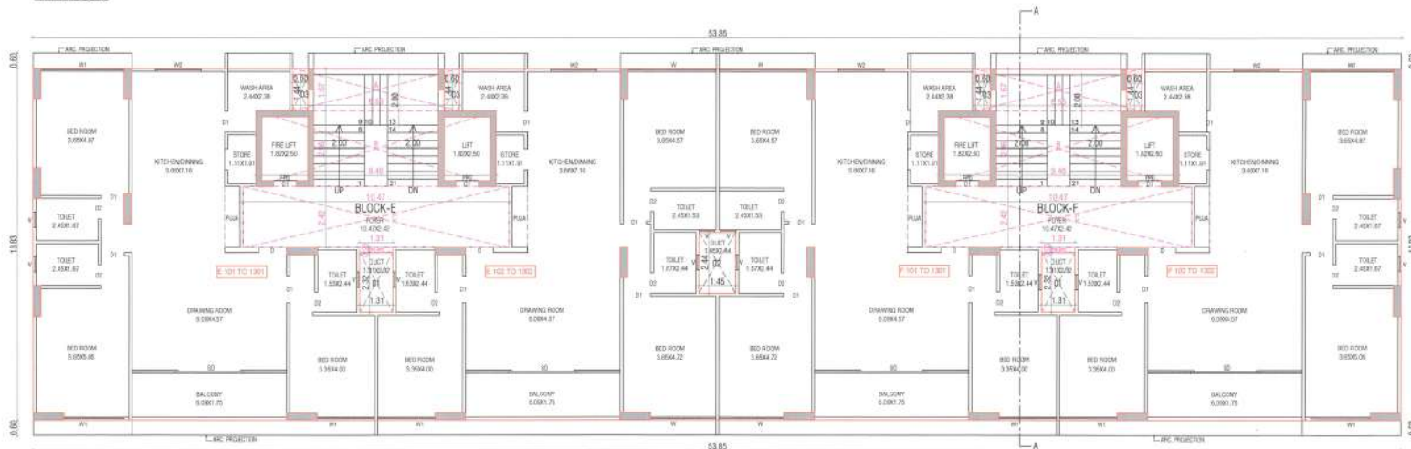
TYPICAL FLOOR PLAN (1st. FLOOR TO 13th. FLOOR)
