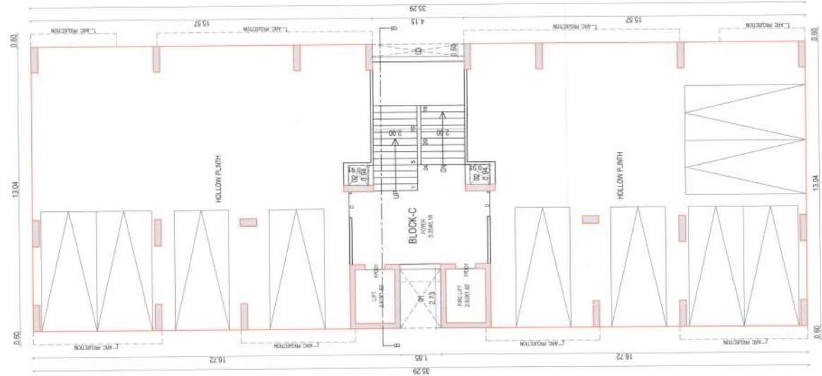
GROUND FLOOR PLAN (HOLLOW PLINTH) BLOCK - C
