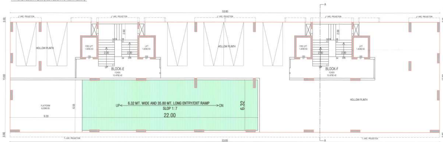
GROUND FLOOR PLAN (HOLLOW PLINTH) BLOCK - E & F
