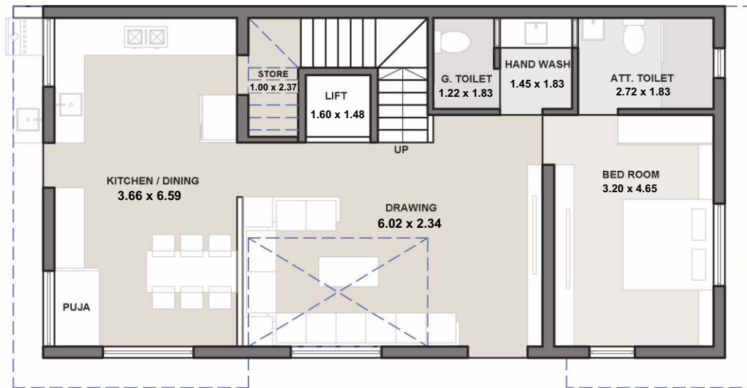
GROUND FLOOR UNIT PLAN
