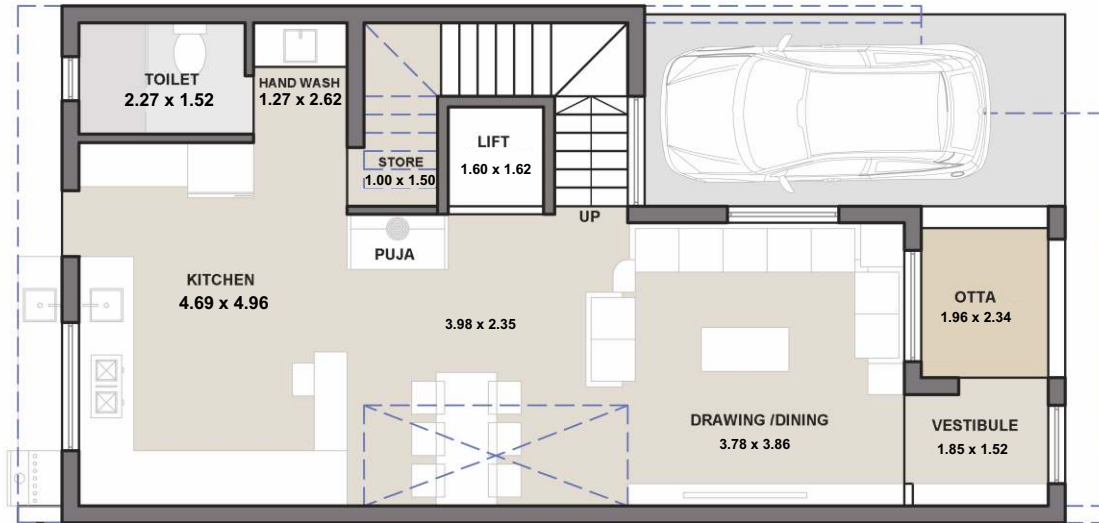
GROUND FLOOR UNIT PLAN
