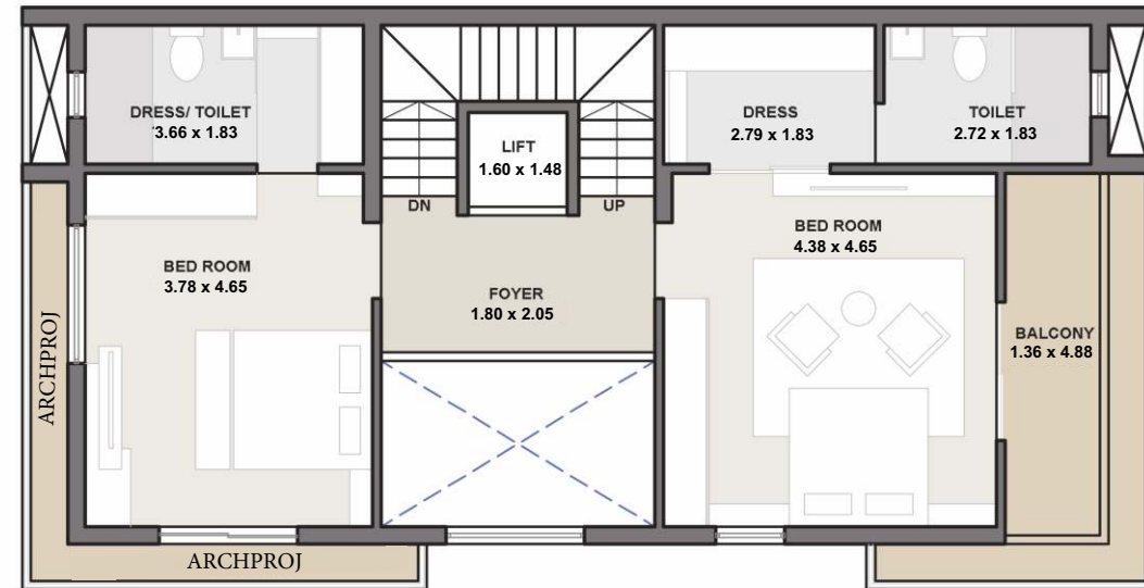
FIRST FLOOR UNIT PLAN
