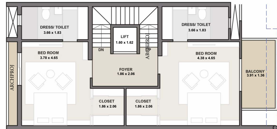
SECOND FLOOR UNIT PLAN
