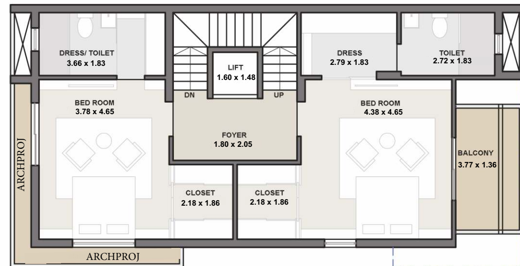
SECOND FLOOR UNIT PLAN
