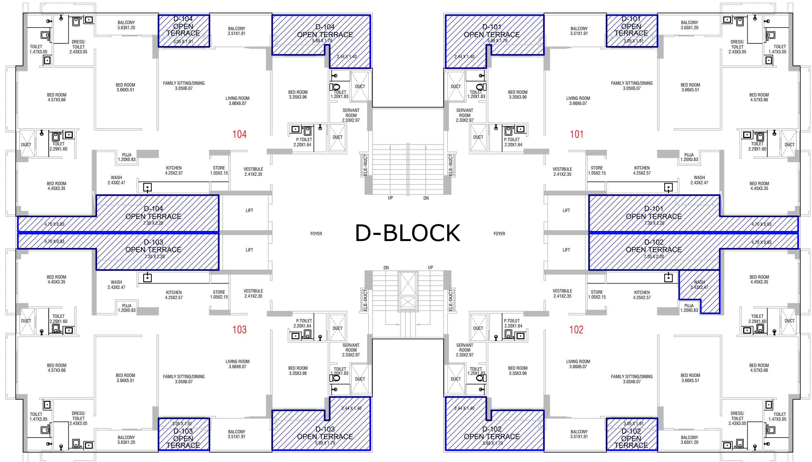
1ST FLOOR PLAN WITH OPEN TERRACE
