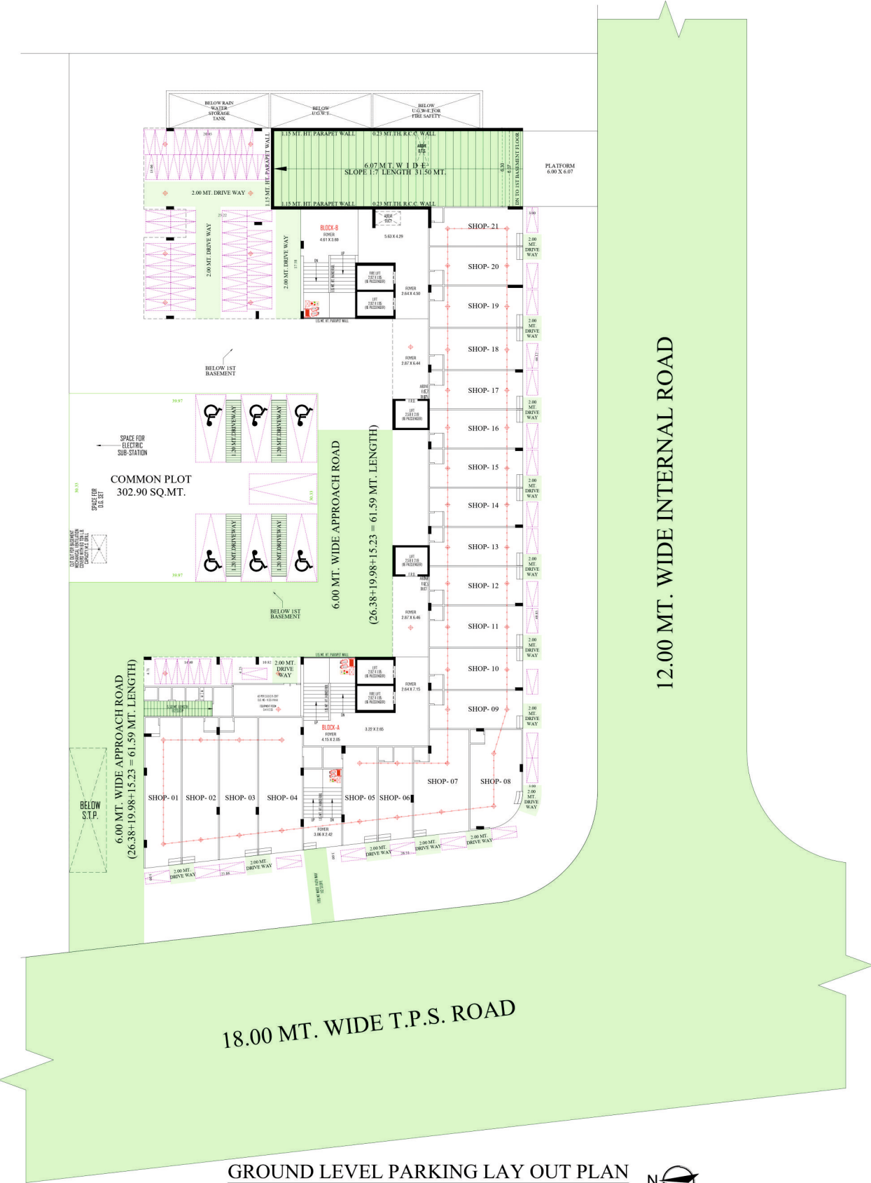
GROUND LEVEL PARKING LAY OUT PLAN [SCALE :- 1.00 CM. = 2.00 MT.]
