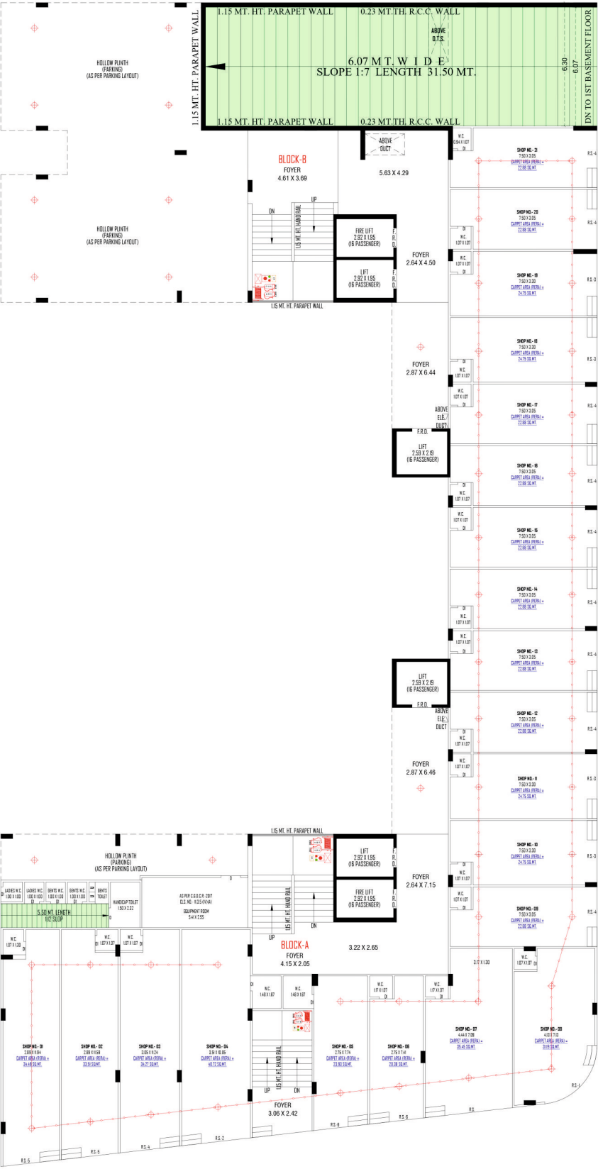
GROUND FLOOR PLAN (SOLID PLINTH+HOLLOW PLINTH) BLOCK:- A+B
