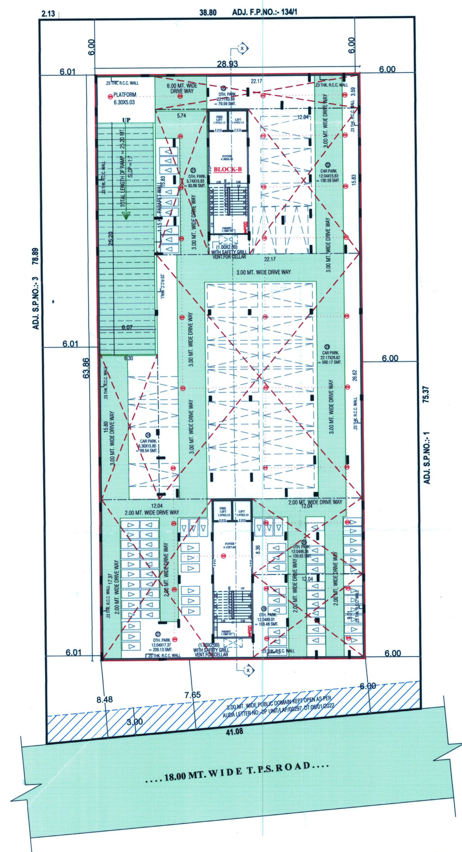
2ND BASEMENT PLAN WITH PARKING LAYOUT
