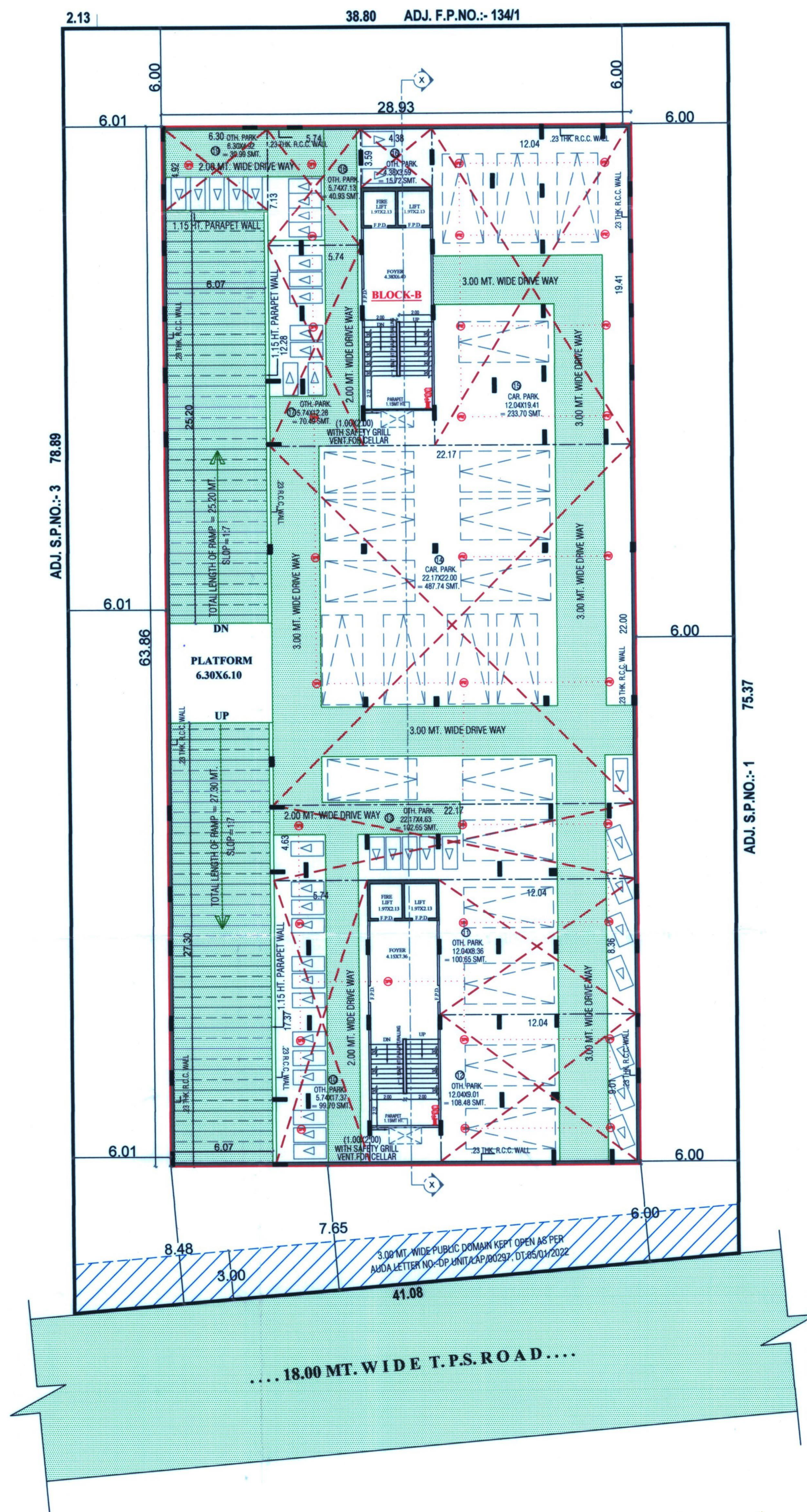
1ST BASEMENT PLAN WITH PARKING LAYOUT
