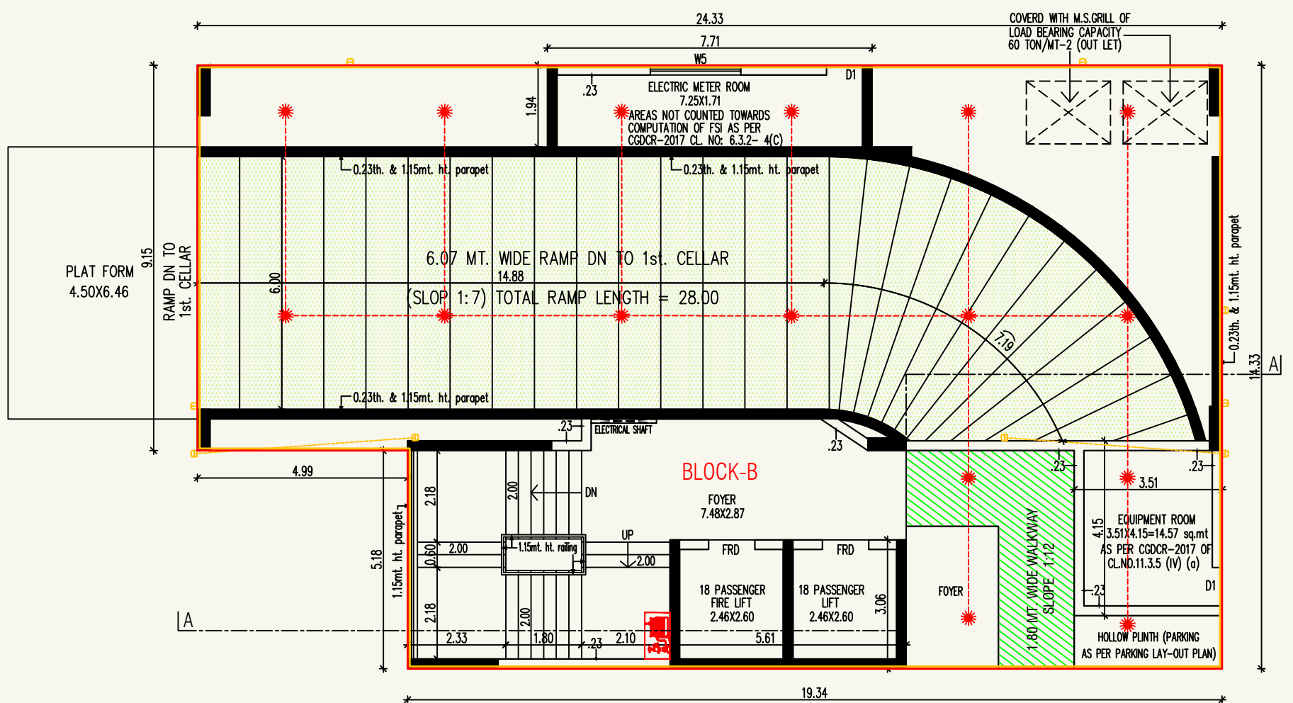
GROUND FLOOR PLAN (HOLLOW PLINTH) (BLOCK-B)
