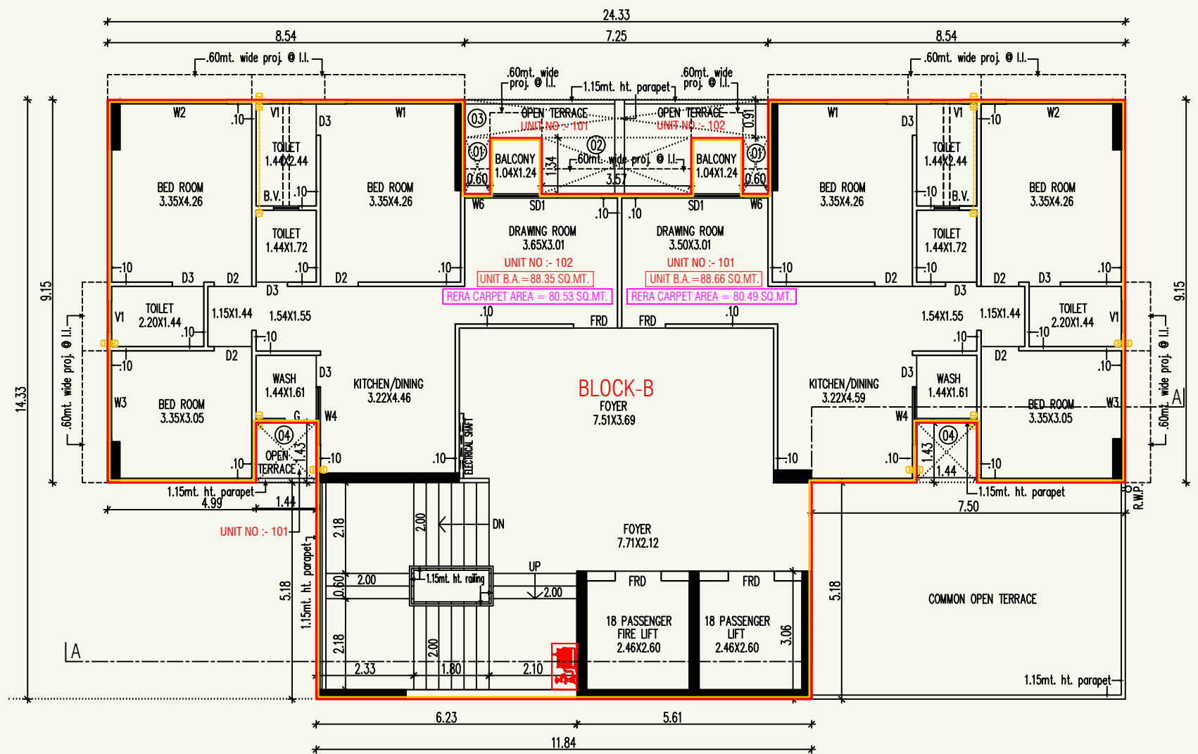
1st. FLOOR PLAN (BLOCK-B)
