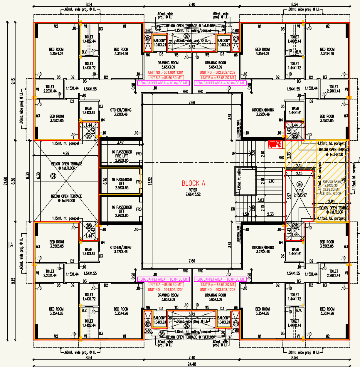
5th., 8th., 12th. FLOOR PLAN (WITH REFUGE AREA) (BLOCK-A)
