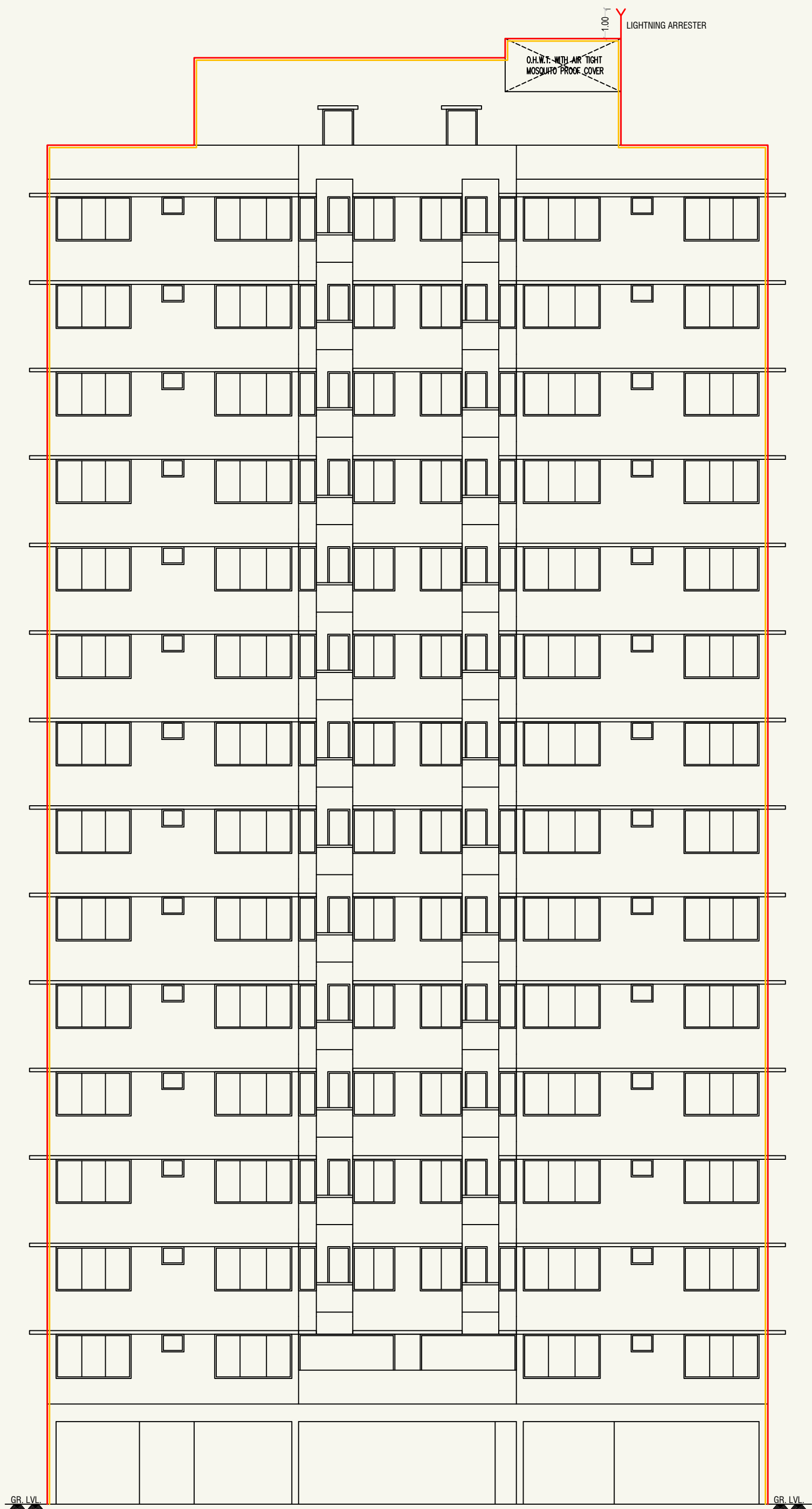
ELEVATION (BLOCK-A)
