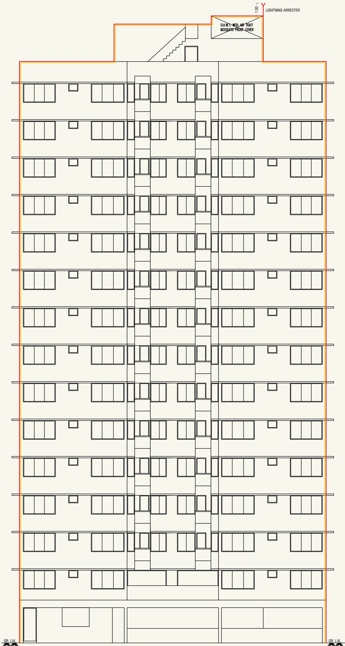
ELEVATION (BLOCK-B)
