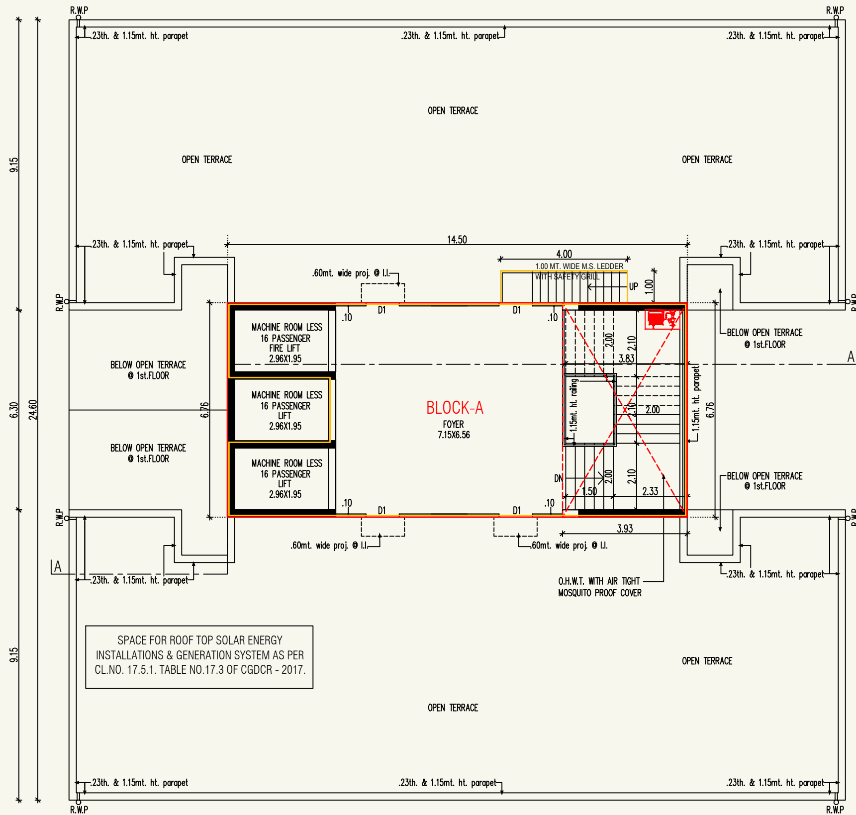
OPEN TERRACE PLAN WITH STAIR CABIN, LMR & O.H.W.T. (BLOCK-A)
