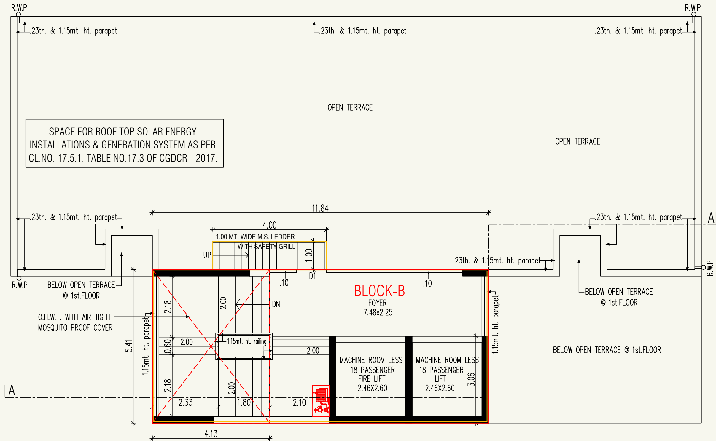
OPEN TERRACE PLAN WITH STAIR CABIN, LMR & O.H.W.T. (BLOCK-B)
