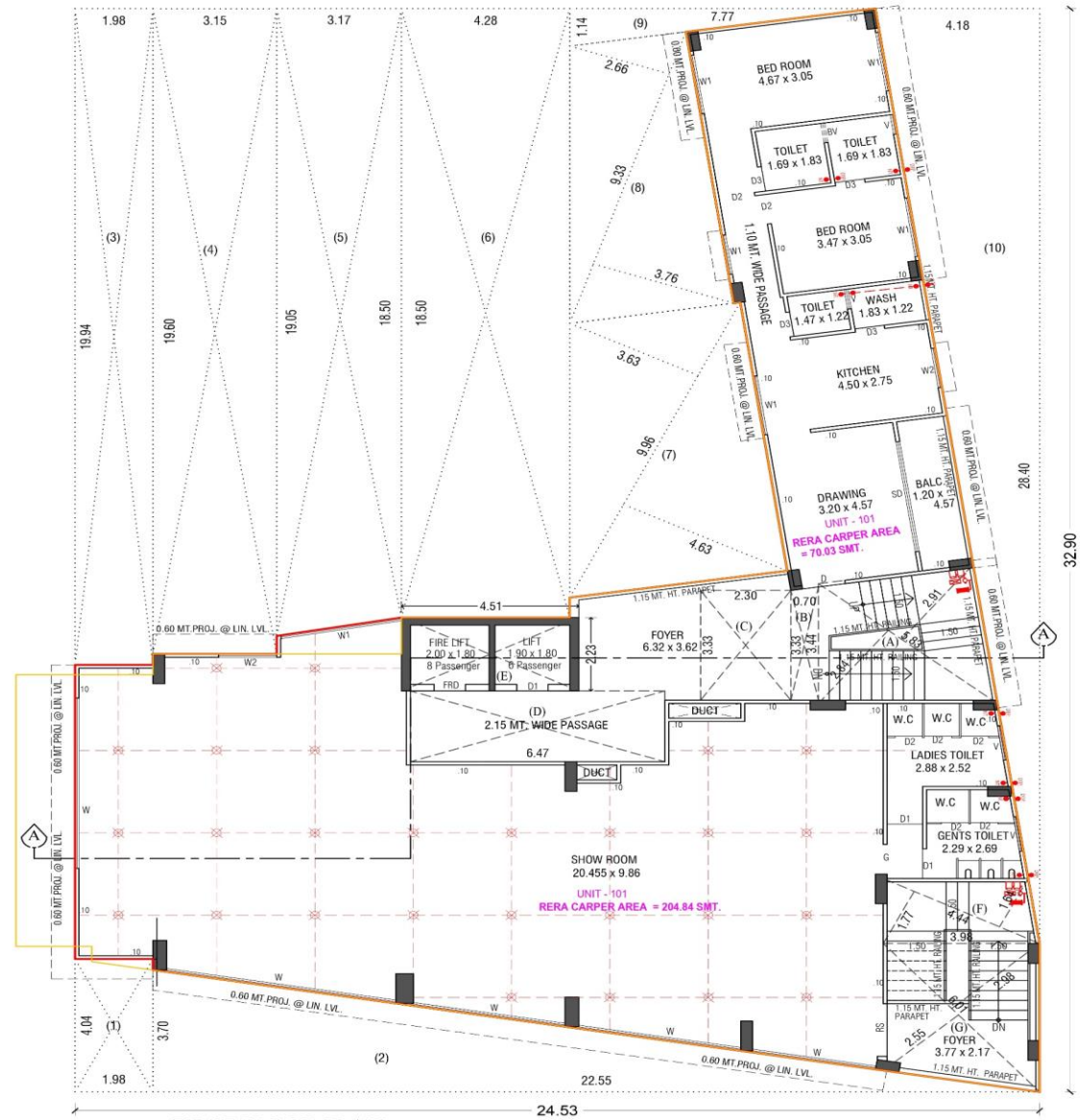
FIRST FLOOR PLAN SCALE :- 1CM = 1MT.
