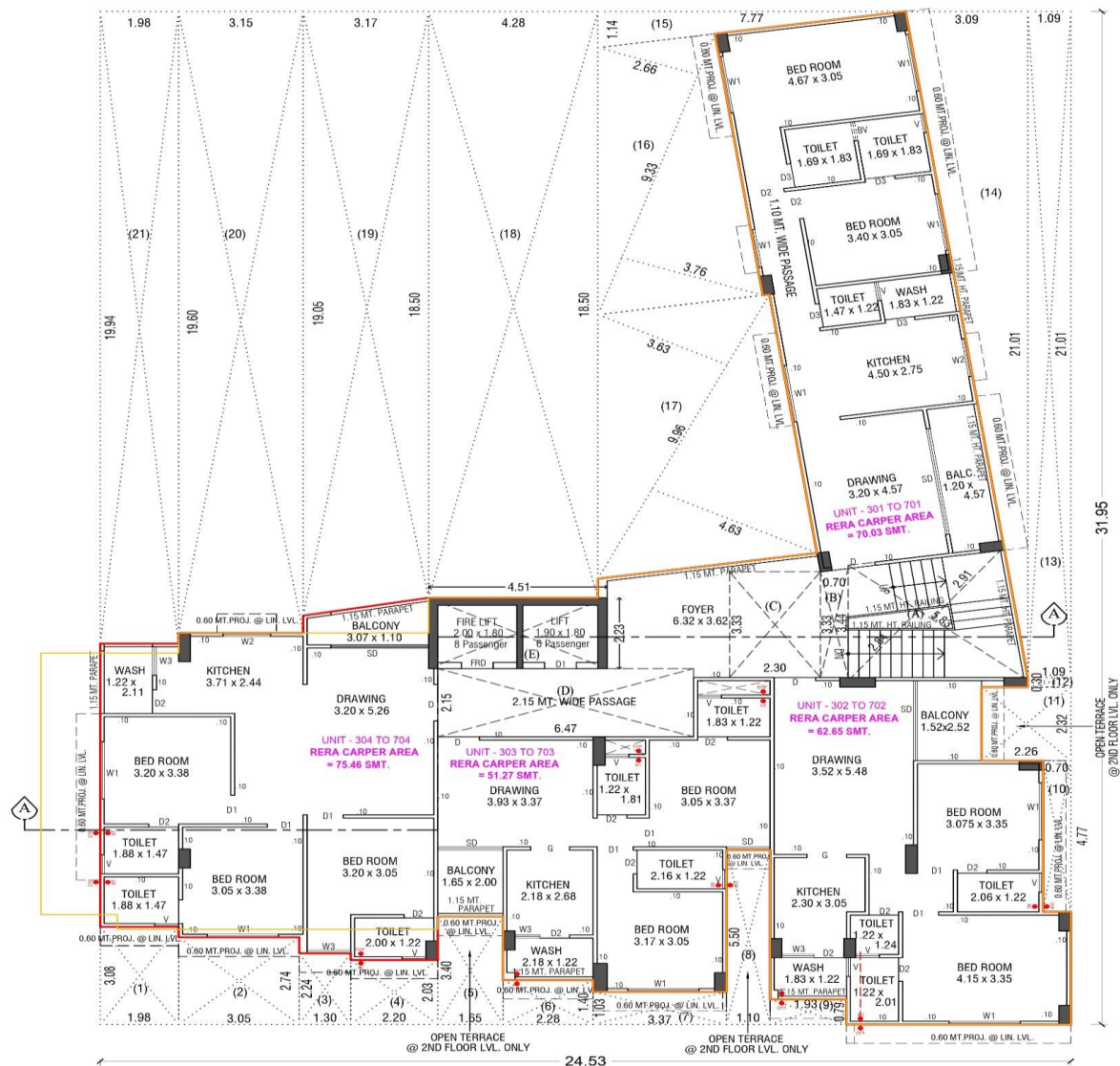
TYPICAL FLOOR PLAN (3RD FLOOR TO 7TH FLOOR) SCALE :- 1CM = 1MT.
