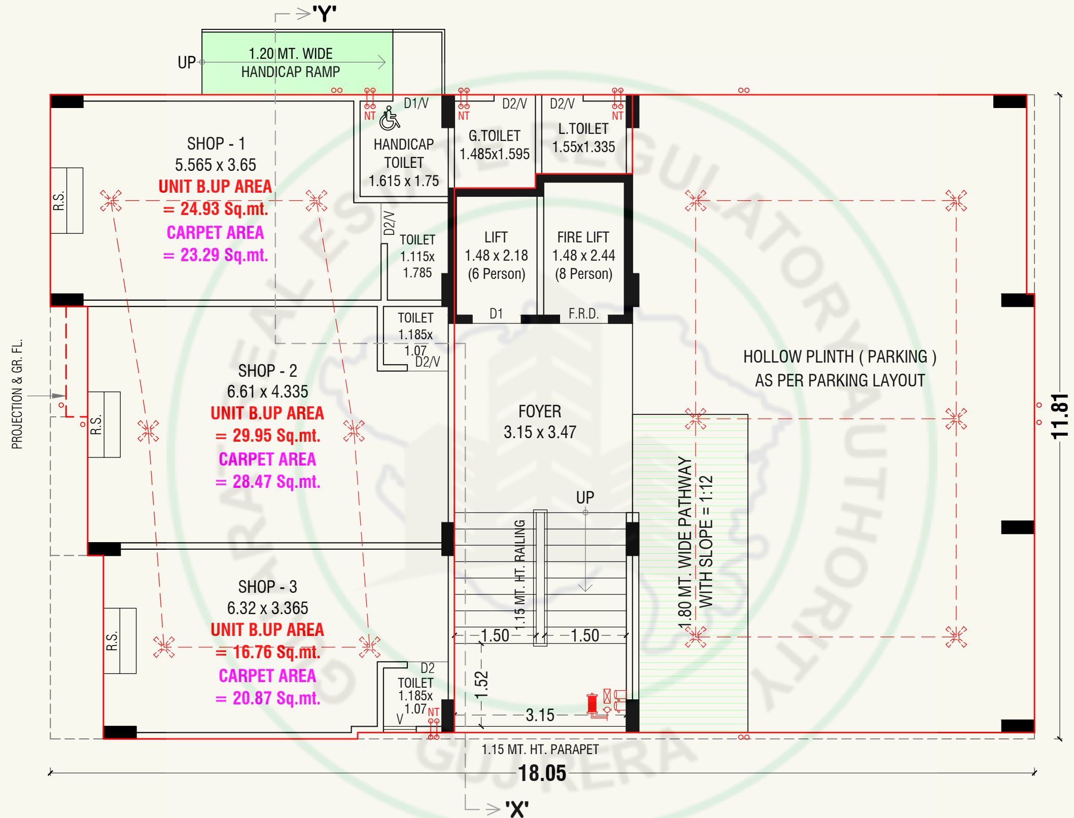
GR. FLOOR PLAN (H.P. PARKING)
