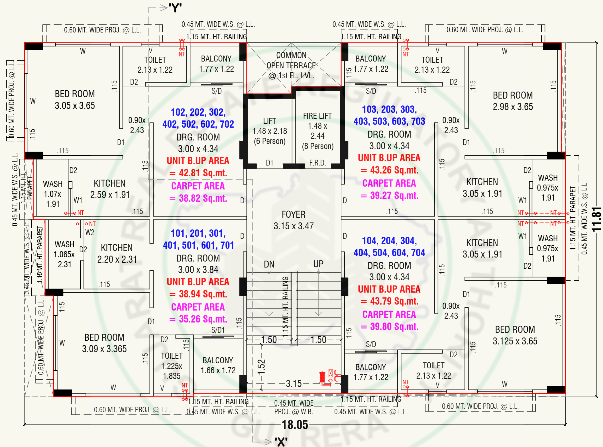
1st to 7th FLOOR PLAN (TYPICAL FL.)
