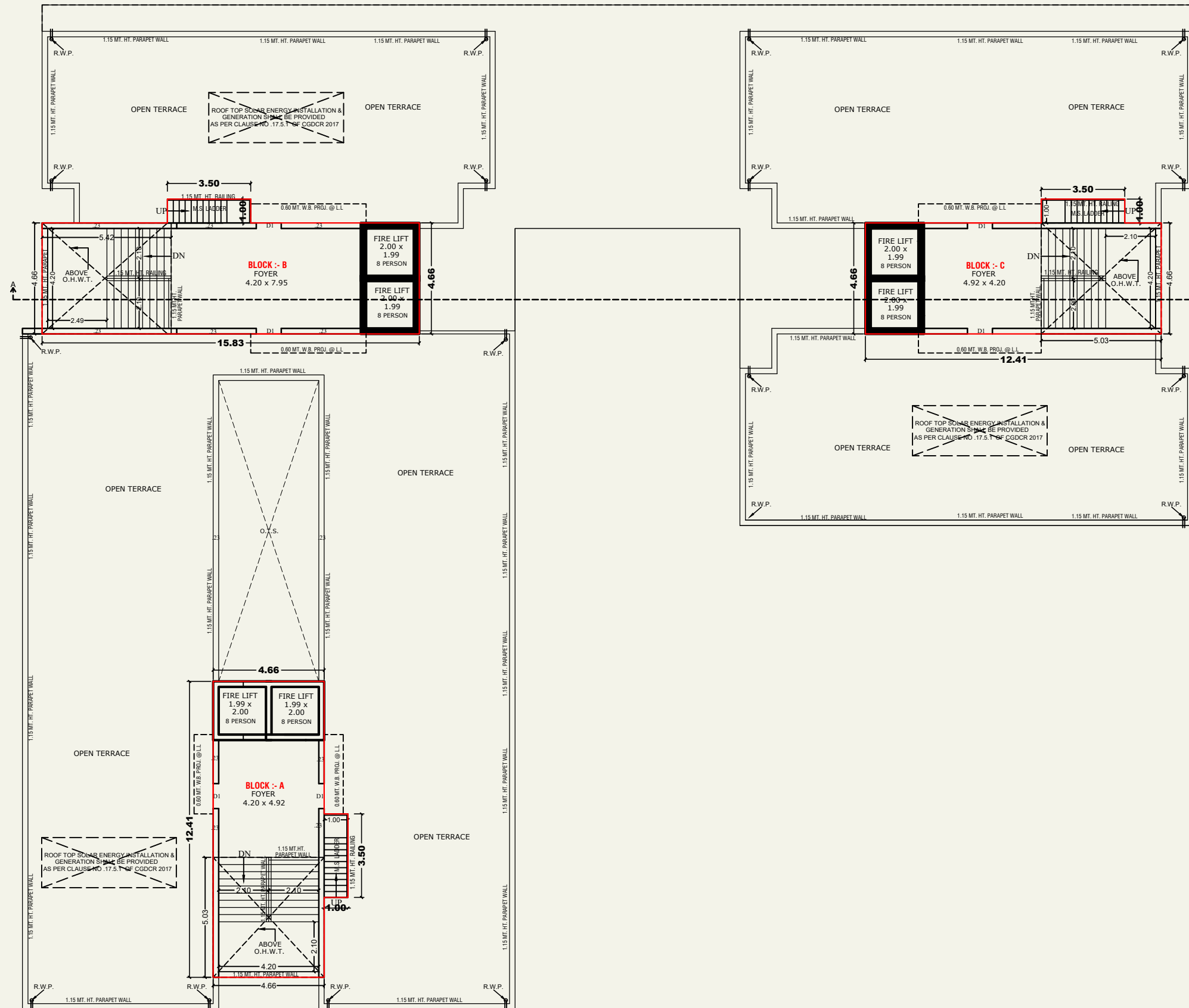
OPEN TERRACE PLAN WITH STAIR CABIN & O.H.W.T.
