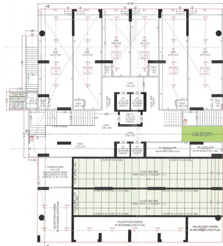
GROUND FLOOR PLAN (PART H.P./PART S.P.)
