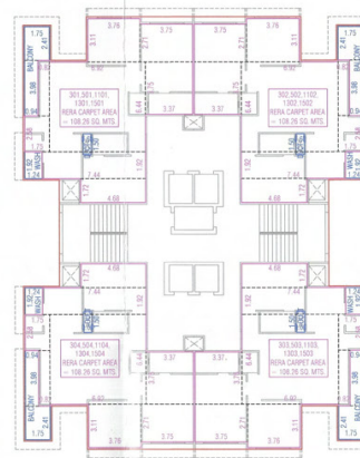
RERA CARPET AREA TYPICAL FLOOR PLAN [3RD, 11TH, 13TH & 15TH FLOOR]
