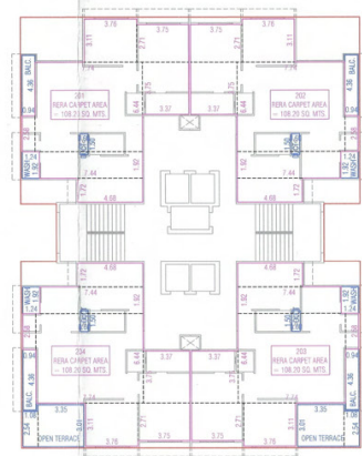
RERA CARPET AREA 2ND FLOOR PLAN
