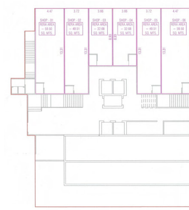
RERA CARPET AREA GROUND FLOOR PLAN
