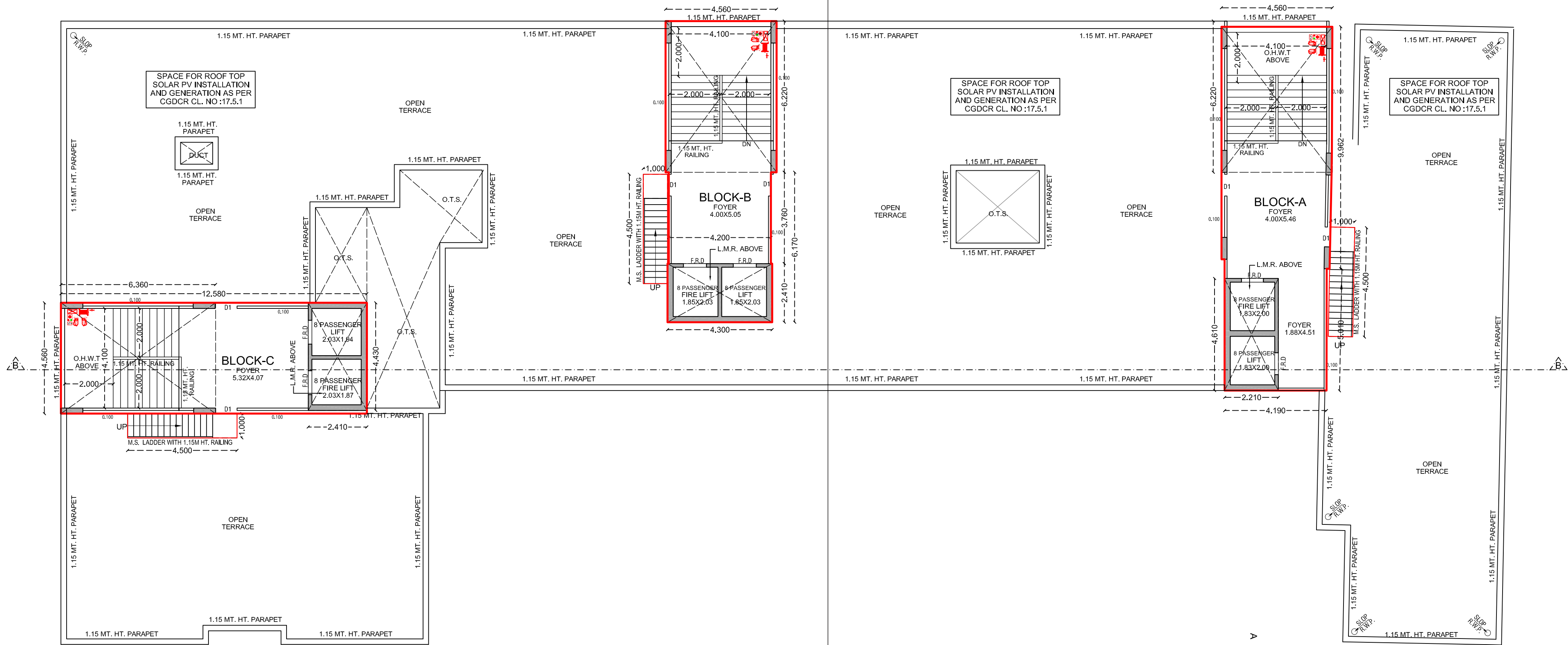
TERRACE PLAN WITH STAIR CABIN, O.H.W.T. & L.M.R
