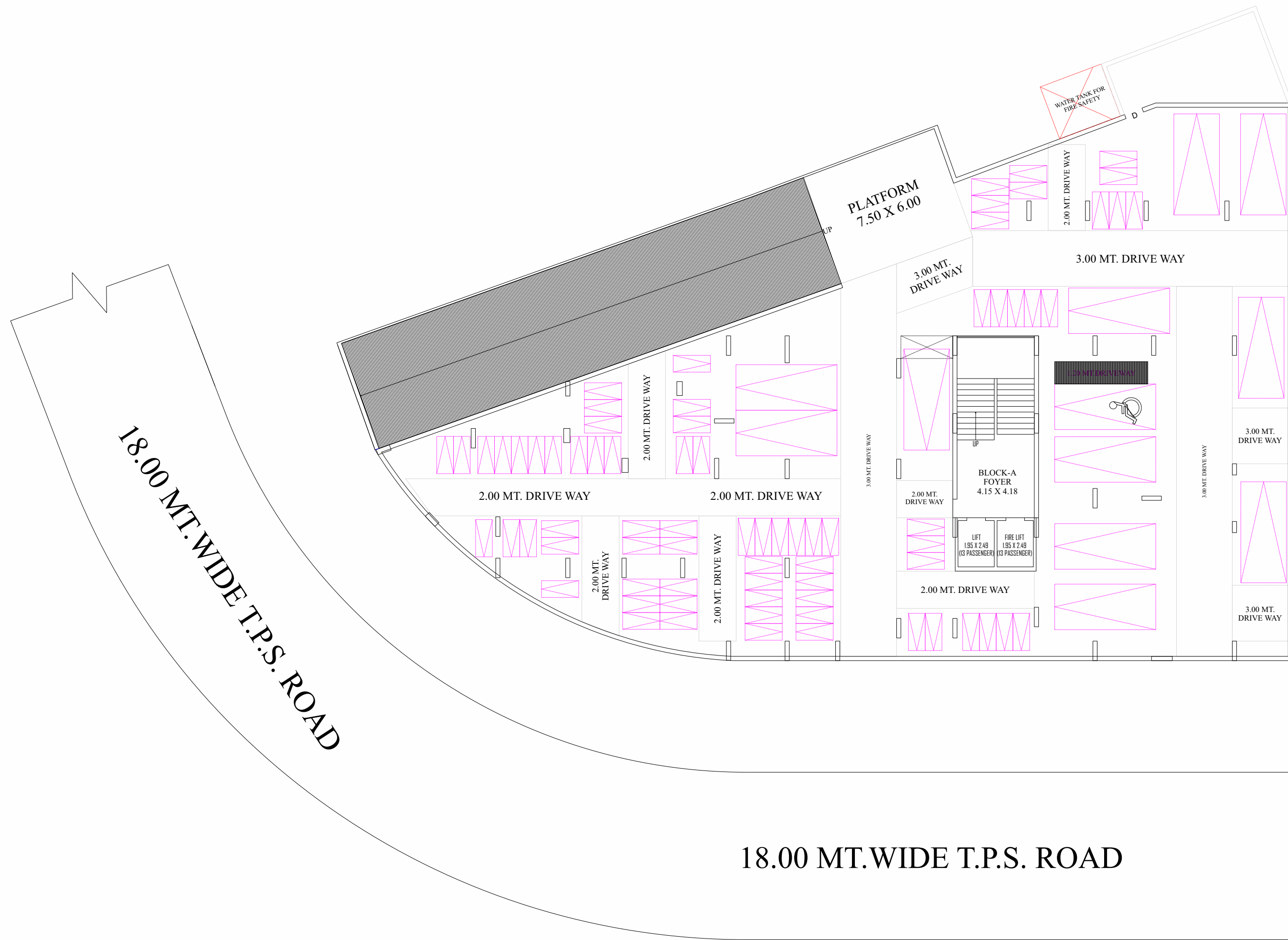
BASEMENT FLOOR LAYOUT PLAN
