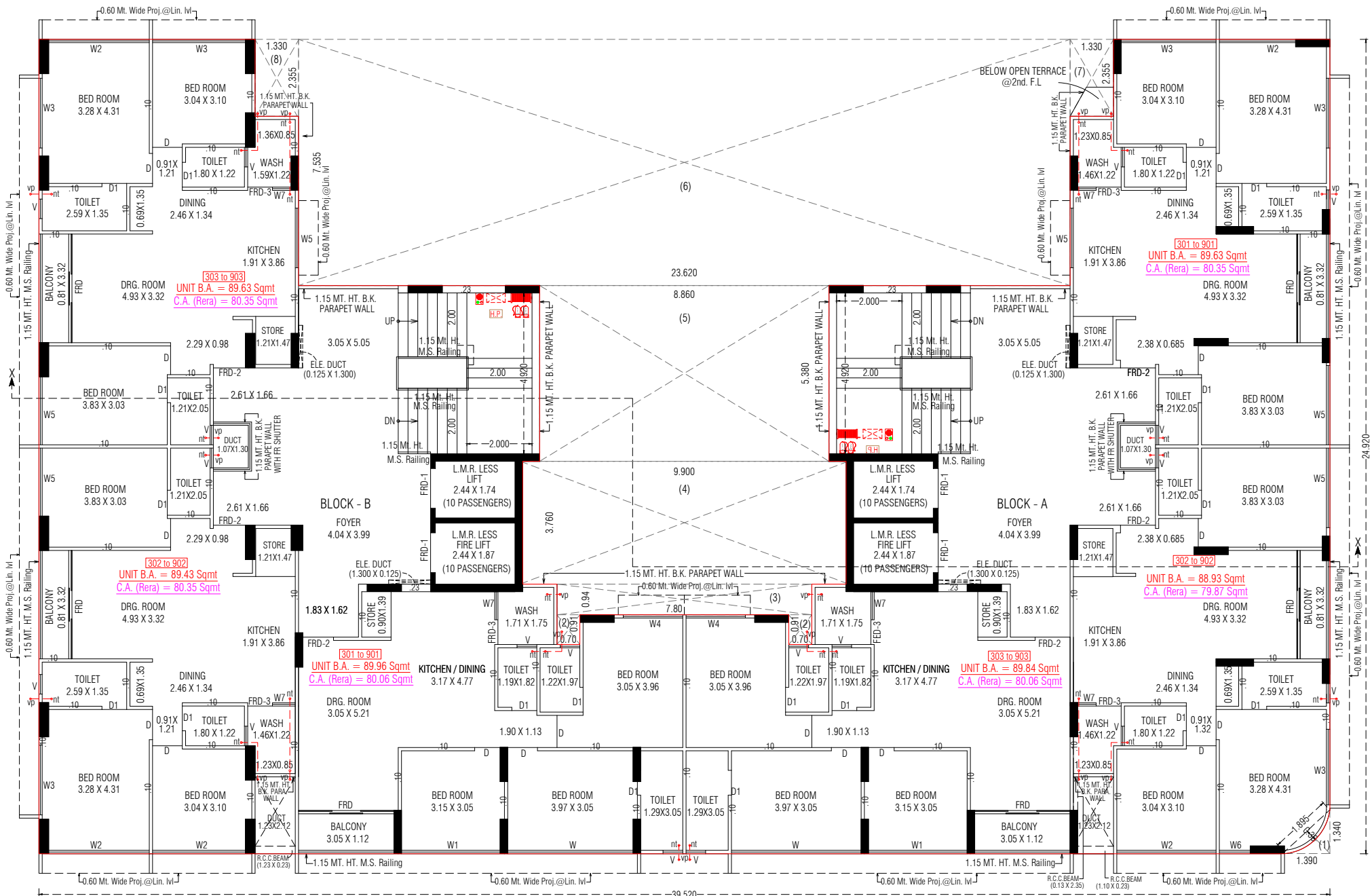
3rd.to 9th. FLOOR PLAN
