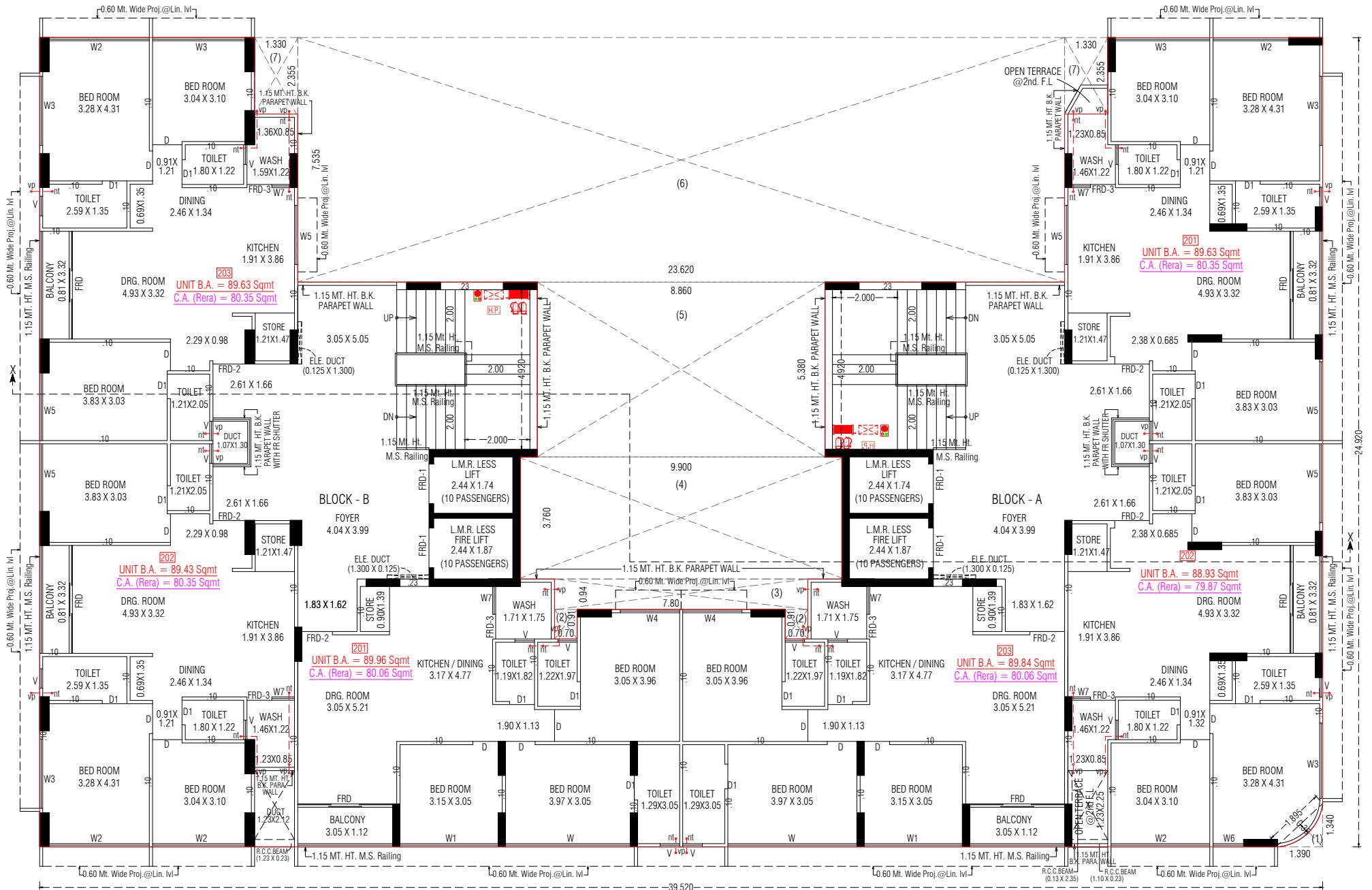
2nd.FLOOR PLAN
