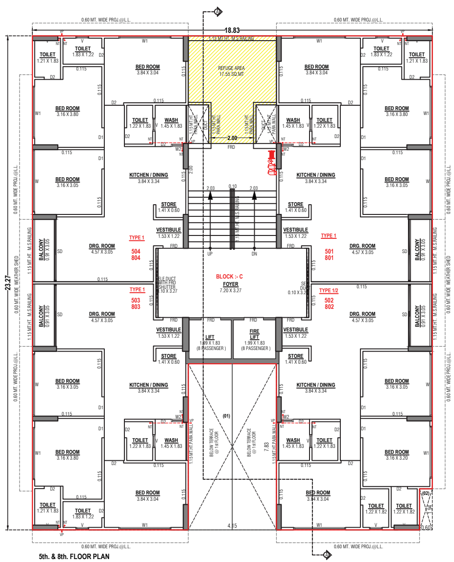
5th. & 8th. FLOOR PLAN
