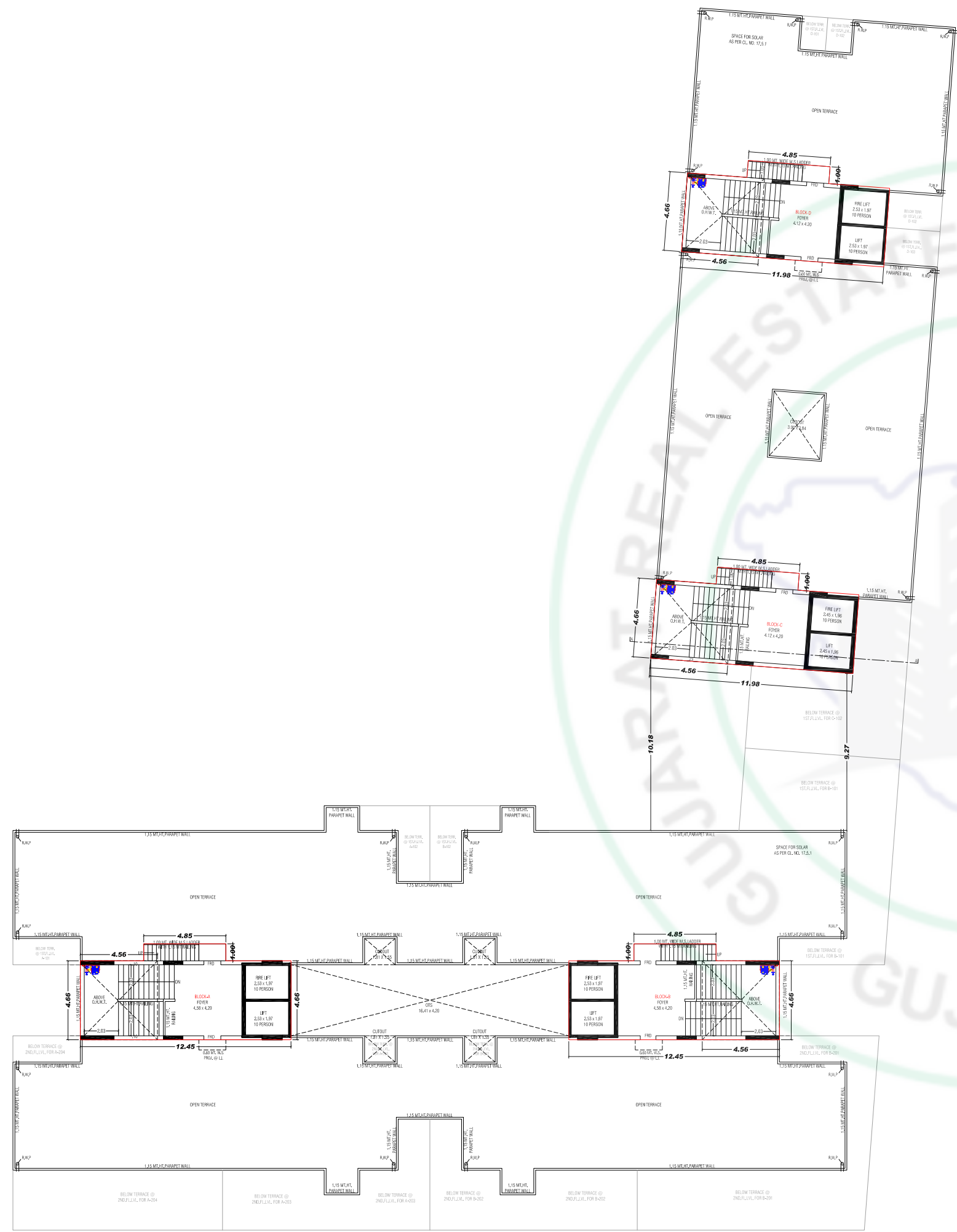
OPEN TERRACE PLAN WITH STAIR CABIN, O.H.W.T.
