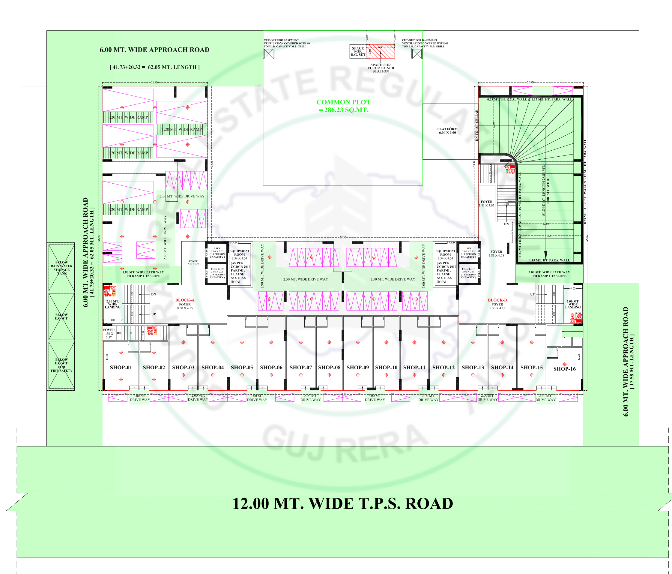
GROUND LEVEL PARKING LAYOUT PLAN
