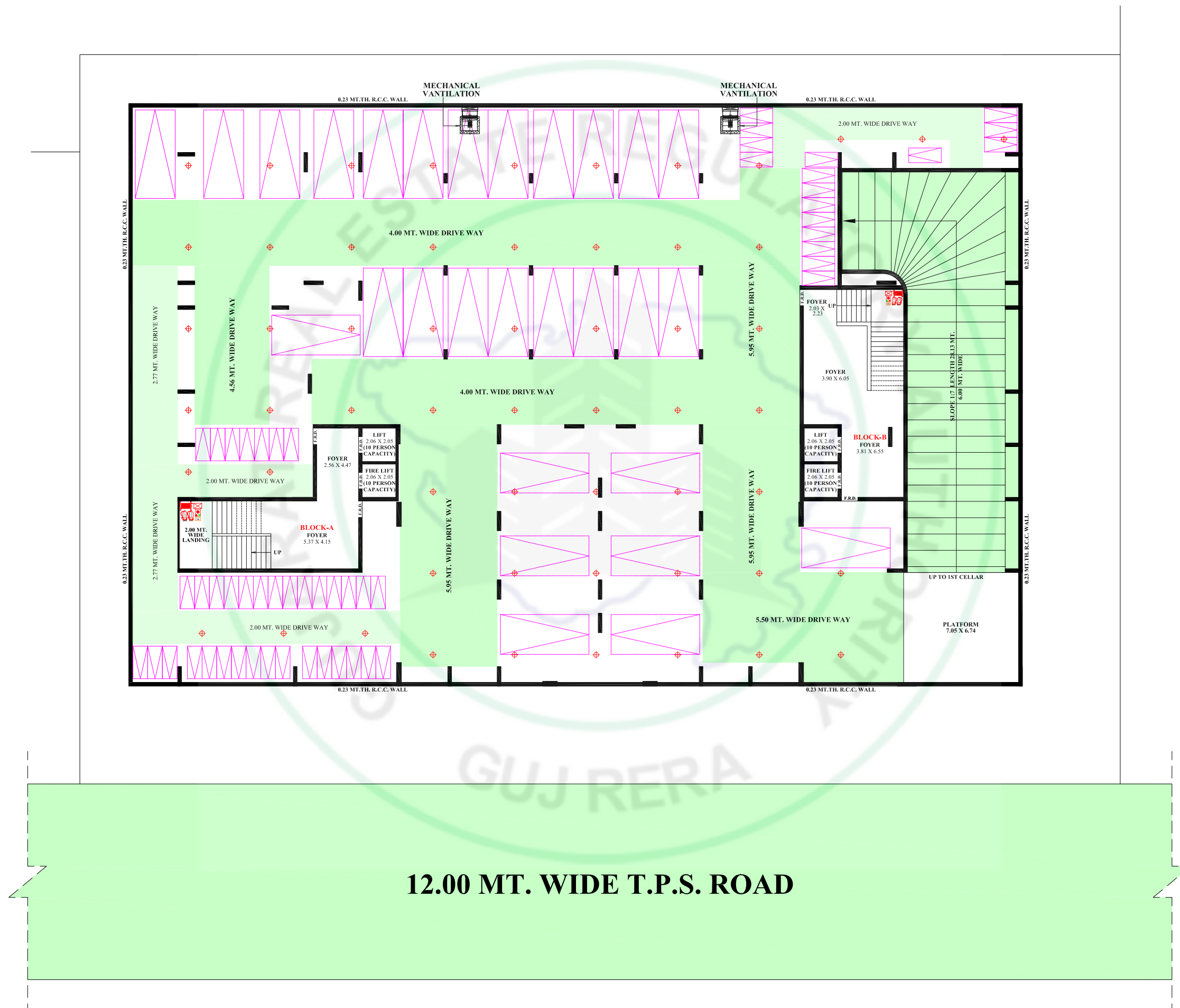
2ND CELLAR PLAN WITH PARKING LAYOUT
