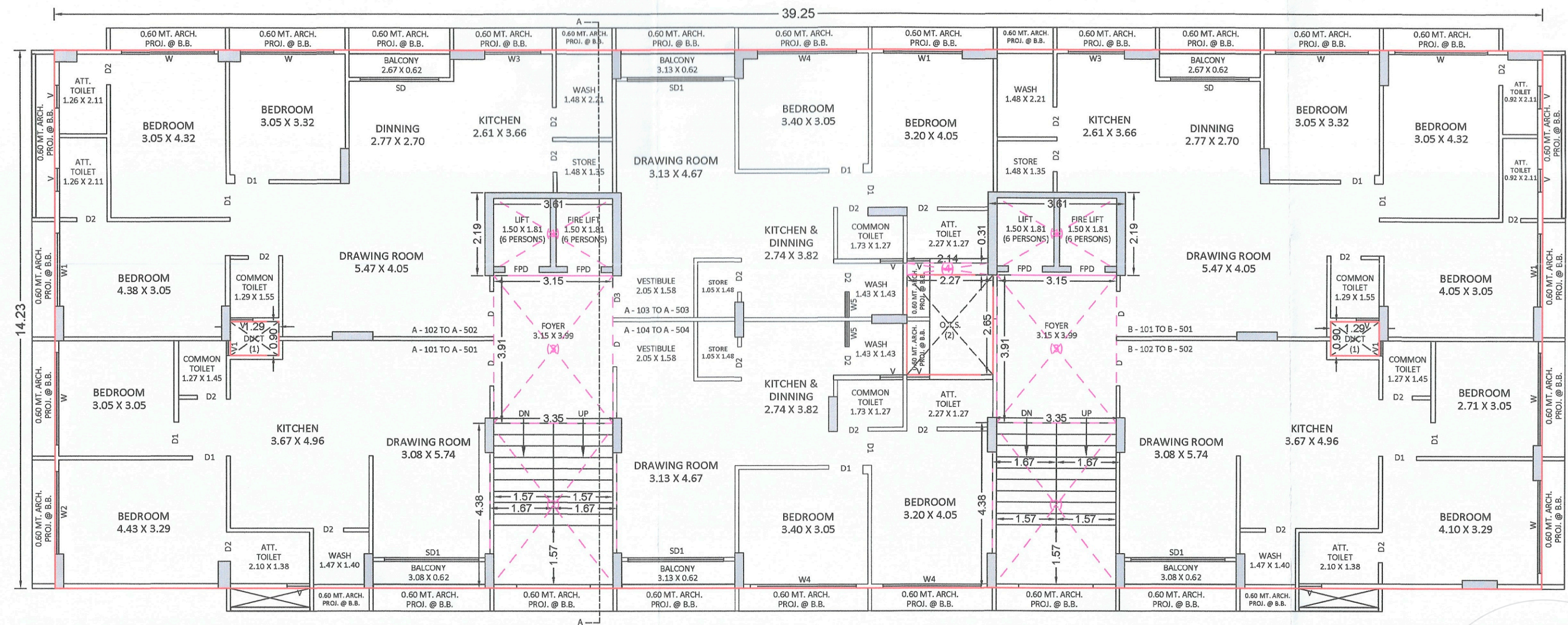
1ST TO 5TH FLOOR PLAN
