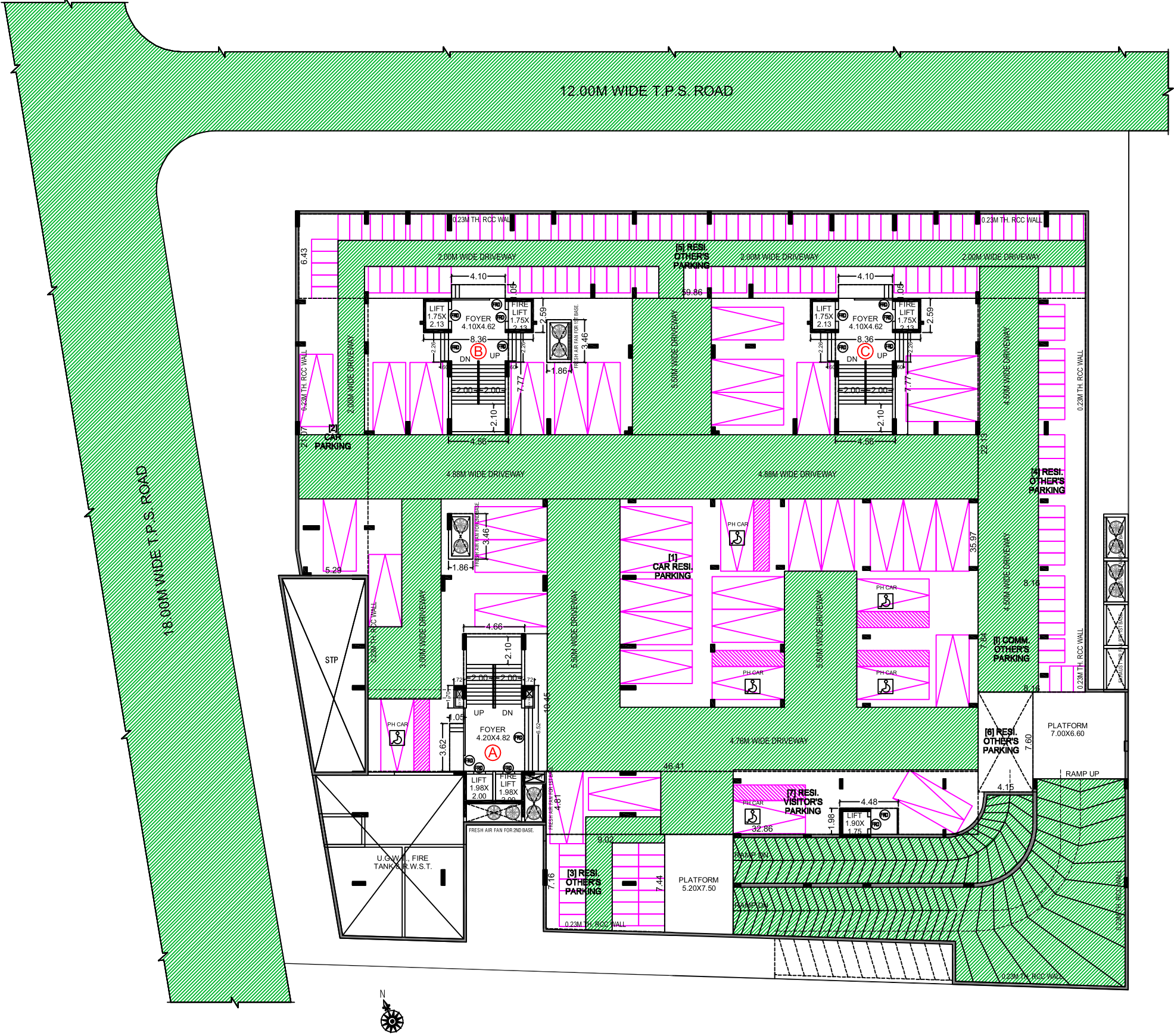
BASEMENT 1 PLAN
