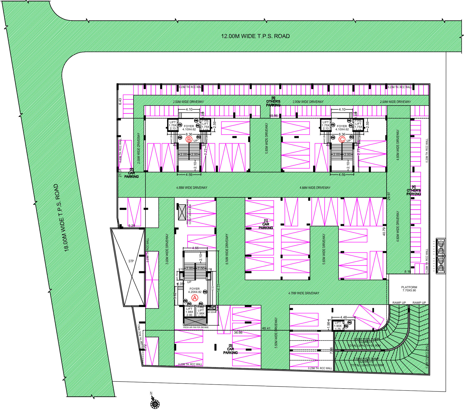
BASEMENT 2 PLAN
