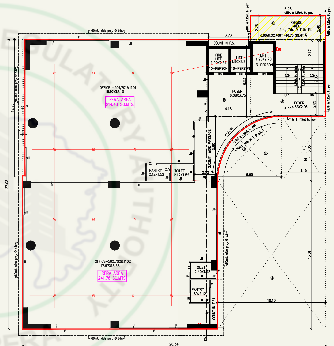
TYPICAL FLOOR PLAN (5th. FL., 7th. FL. & 11th. FL.) (WITH REFUGE AREA)
