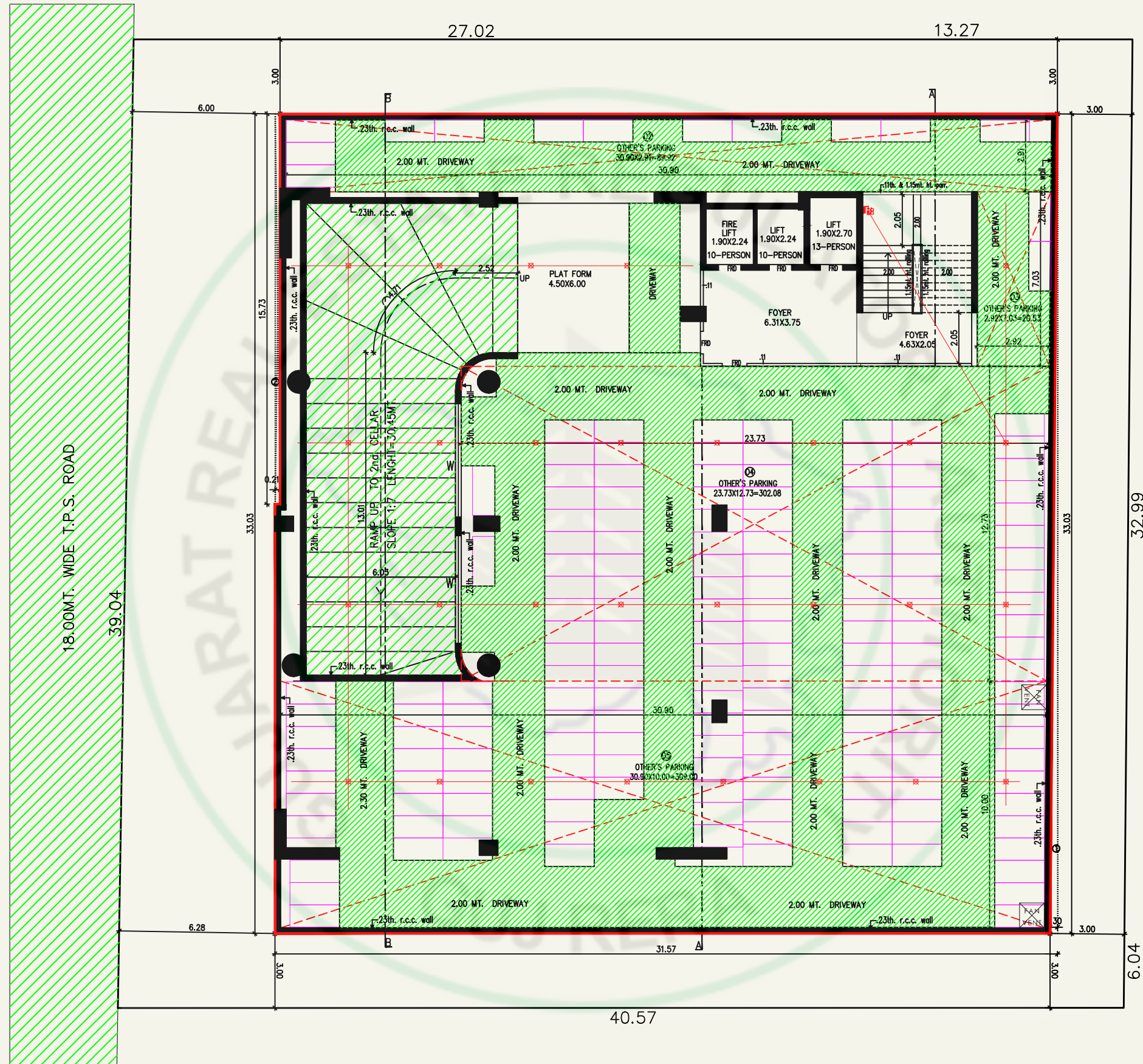
3rd. CELLAR PLAN
