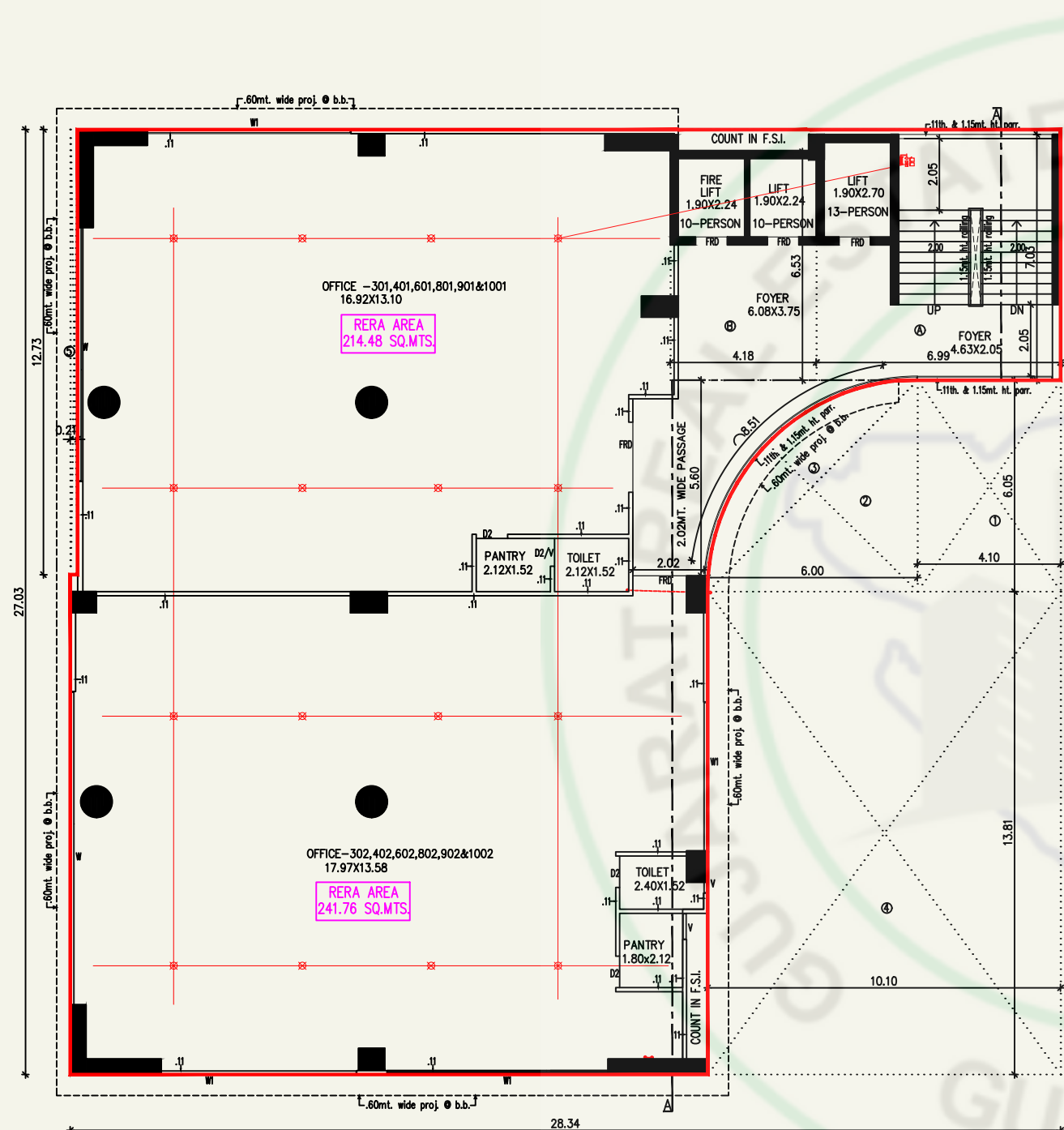
TYPICAL FLOOR PLAN (3rd. FL., 4th. FL., 6th. FL., 8th. FL. TO 10th. FL.)
