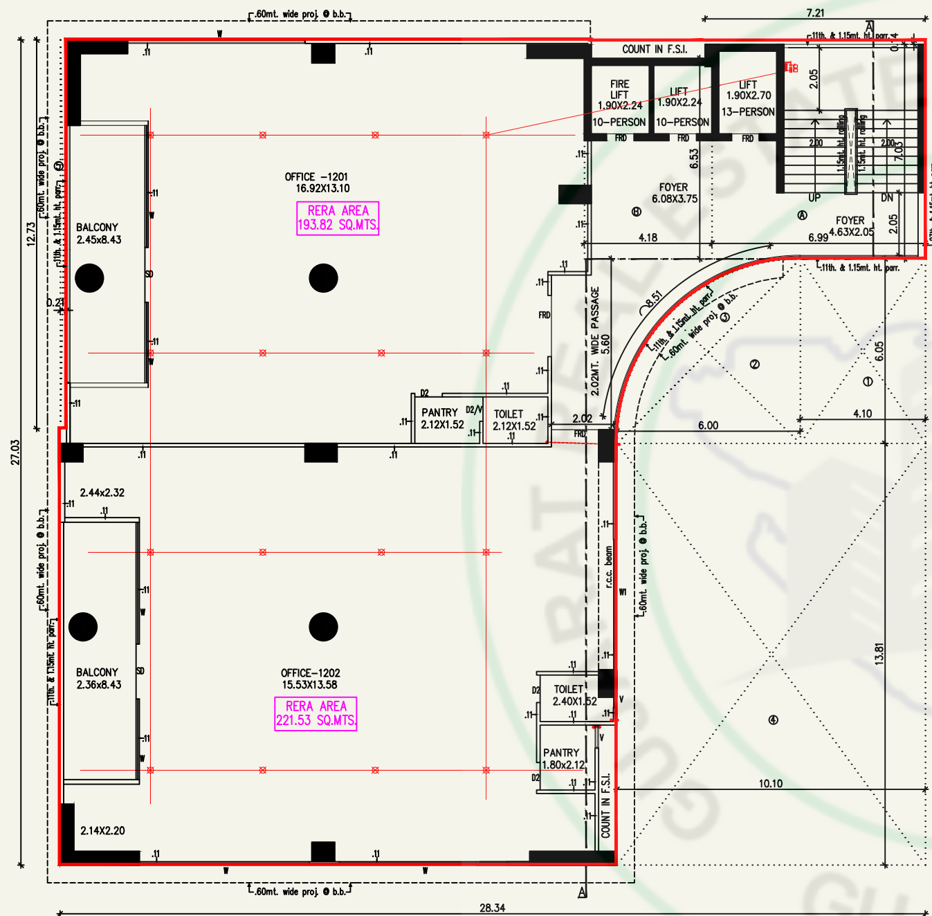
12th. FLOOR PLAN
