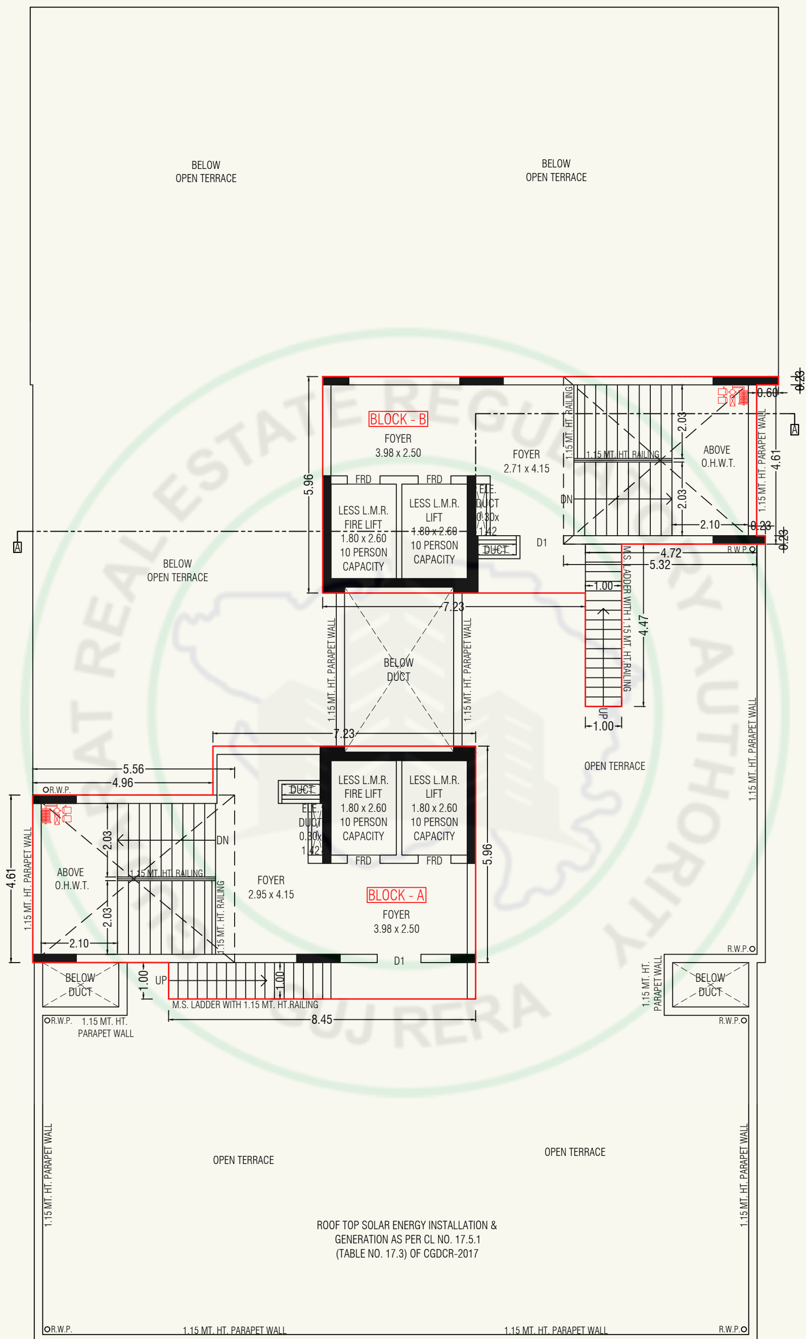
OPEN TERRACE PLAN WITH STAIR CABIN & O.H.W.T.
