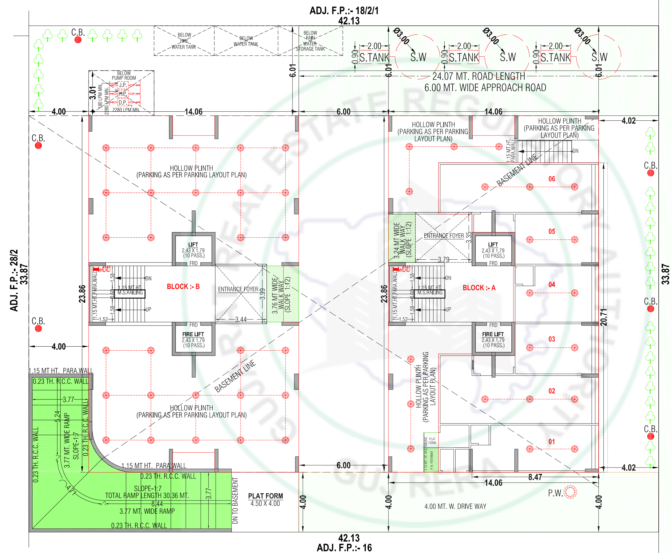
LAYOUT PLAN SCALE : 1 CM = 2.00 MT
