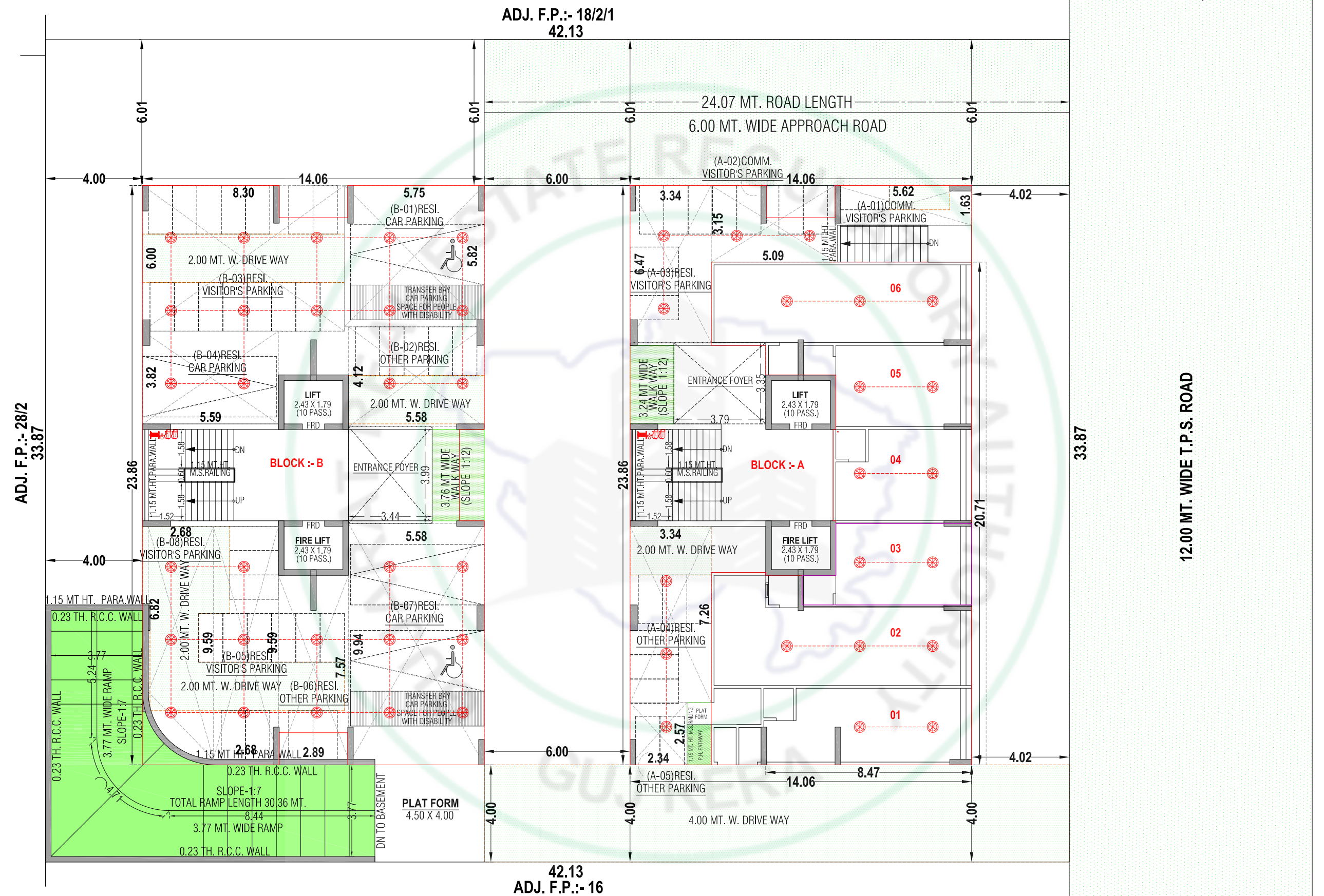
PARKING LAYOUT PLAN SCALE : 1 CM = 2.00 MT
