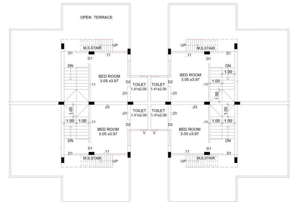
S. FLOOR PLAN & OPEN TERRACE PLAN
