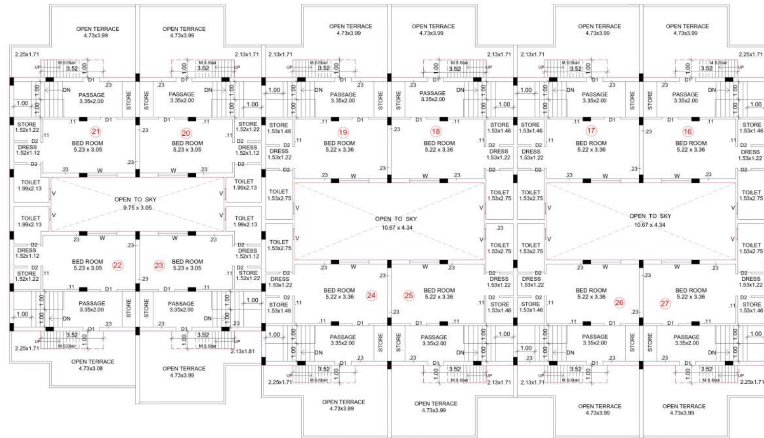
S. FLOOR PLAN & OPEN TERRACE PLAN
