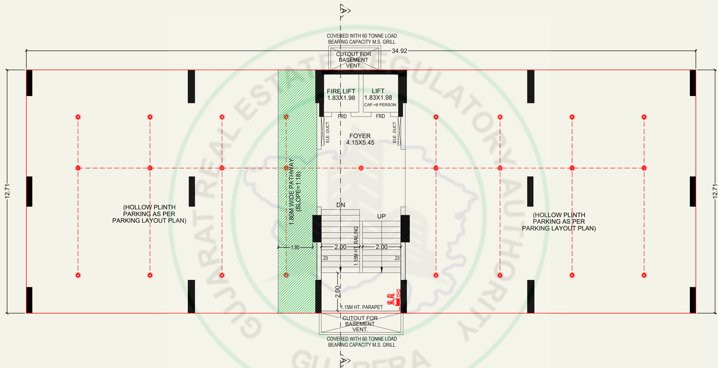
GROUND FLOOR PLAN (HOLLOW PLINTH) (BLOCK-B)
