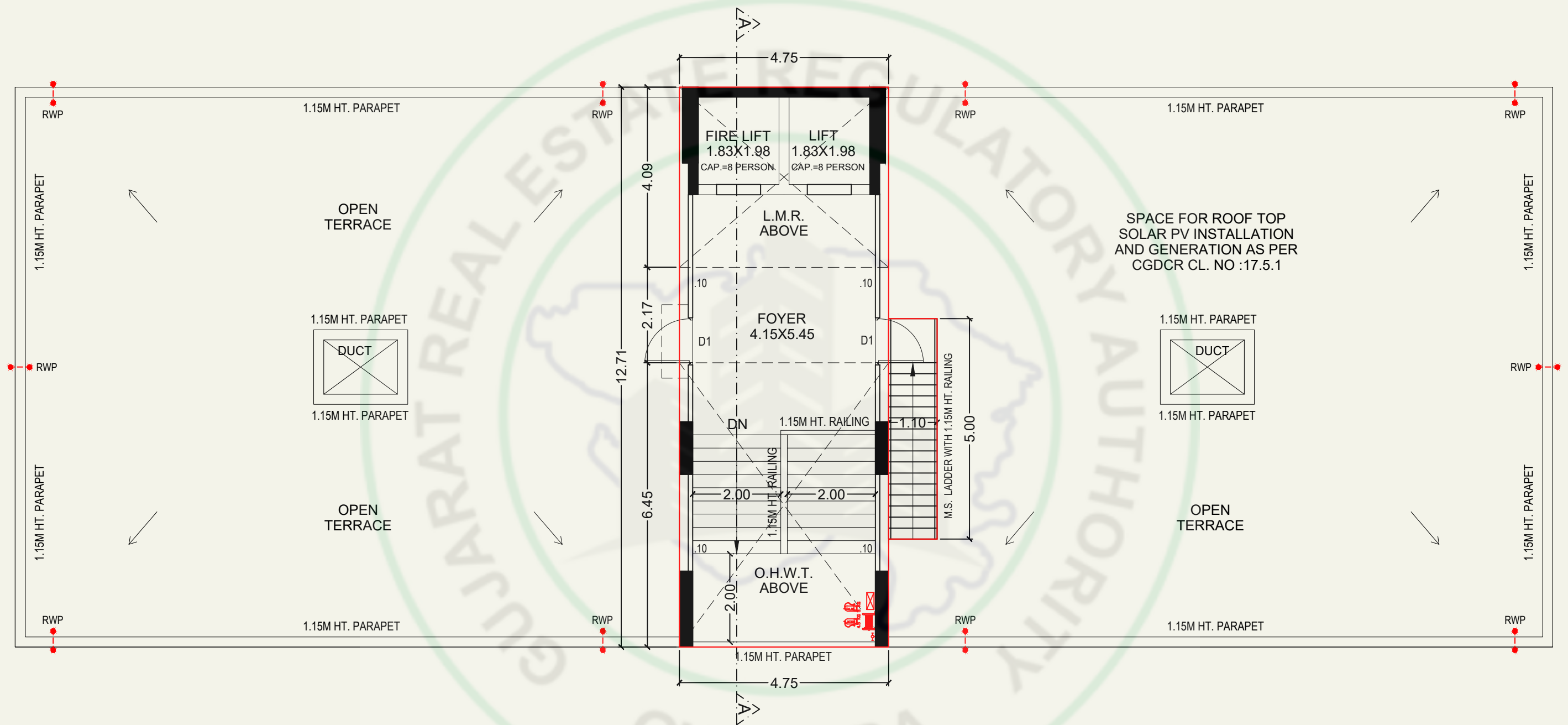
OPEN TERRACE PLAN WITH STAIR CABIN, L.M.R. & O.H.W.T. (BLOCK-B)
