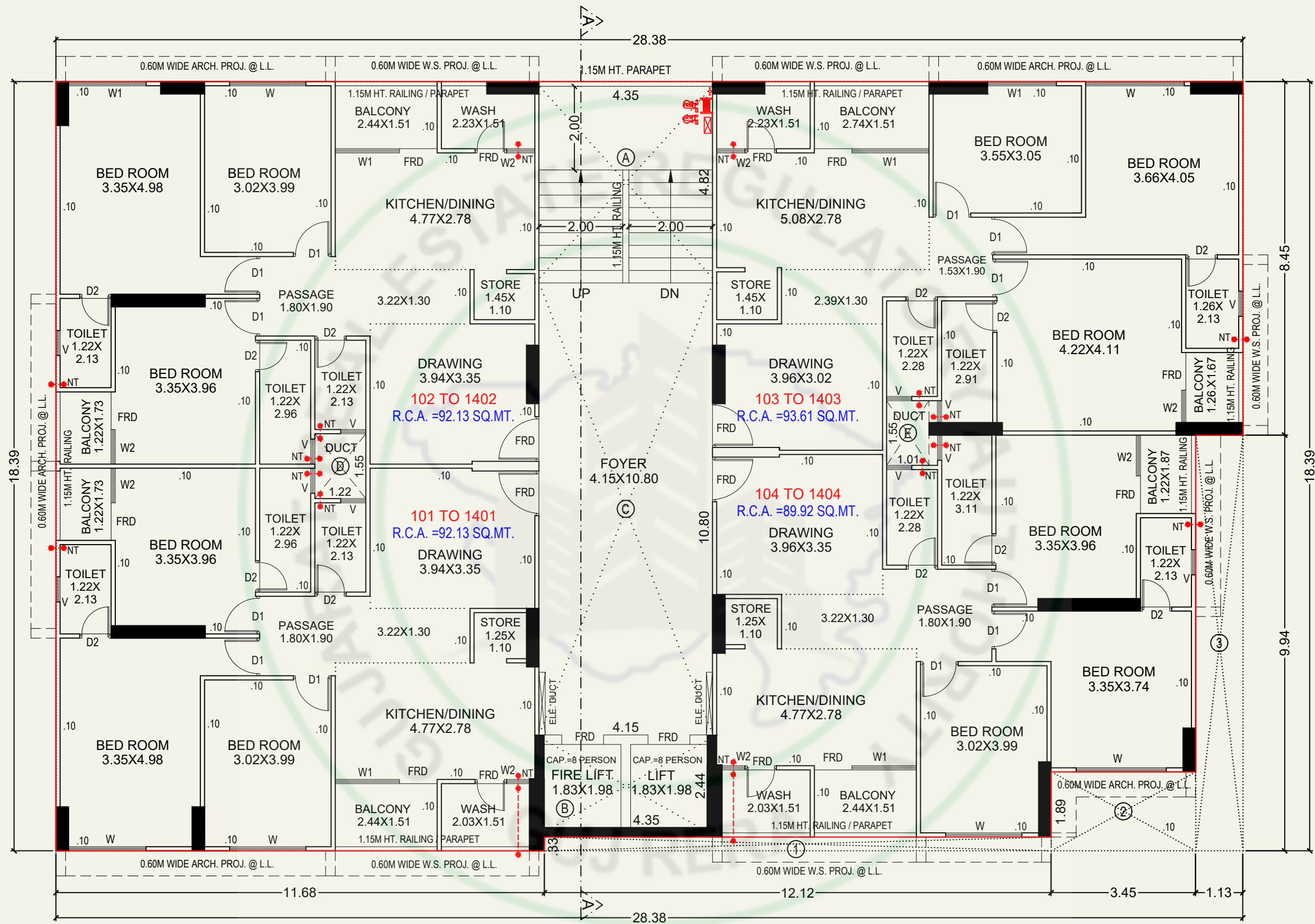
1ST TO 14TH FLOOR PLAN (BLOCK-A)
