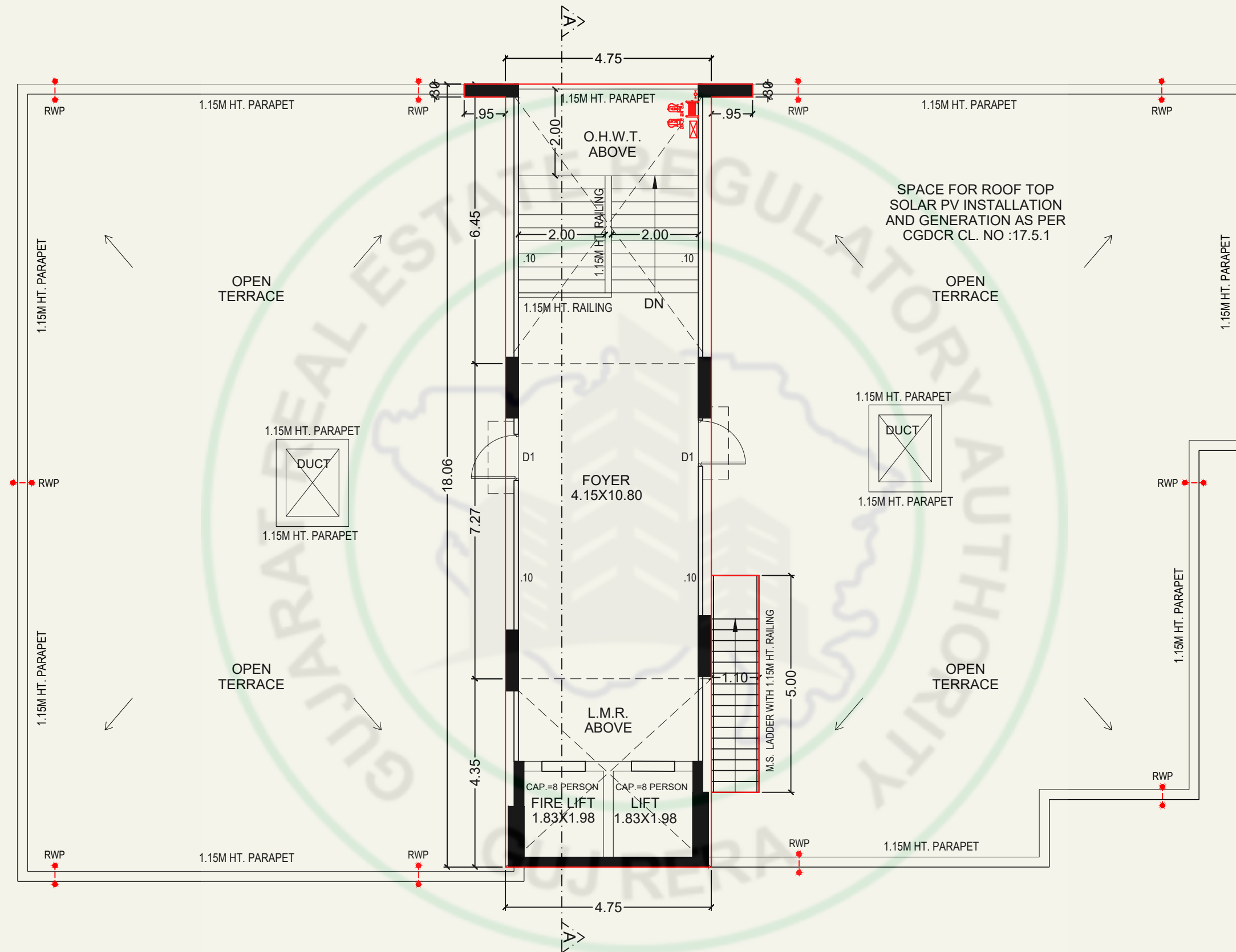
OPEN TERRACE PLAN WITH STAIR CABIN, L.M.R. & O.H.W.T. (BLOCK-A)
