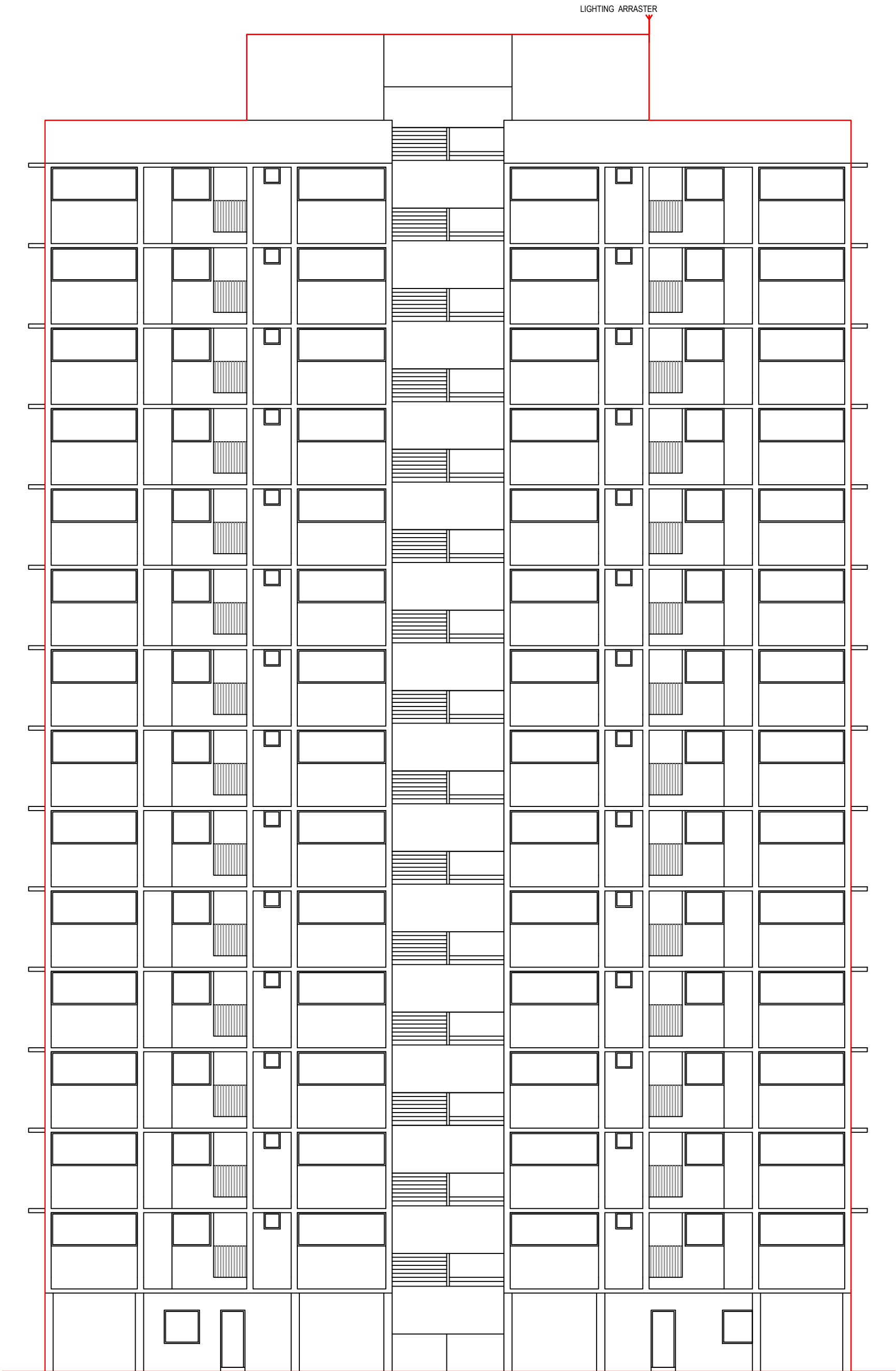
ELEVATION (BLOCK - F)
