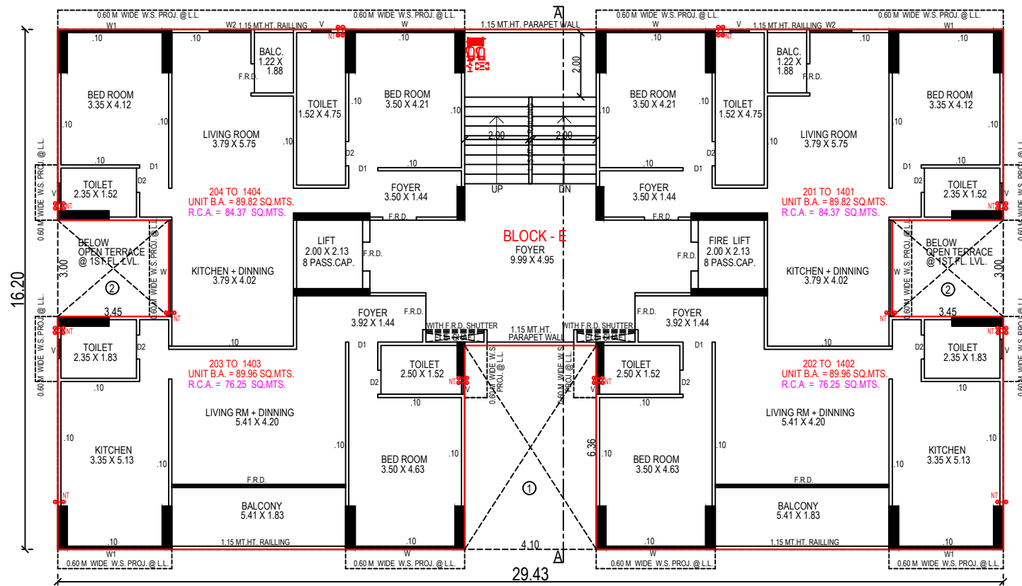
TYPICAL FLOOR PLAN (2ND. TO 14TH. FLOOR PLAN) (BLOCK - E)
