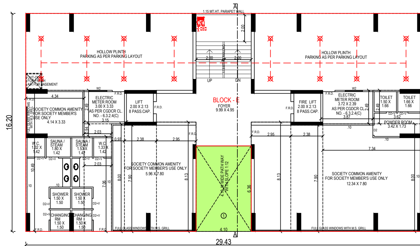
GROUND FLOOR PLAN (BLOCK - E)
