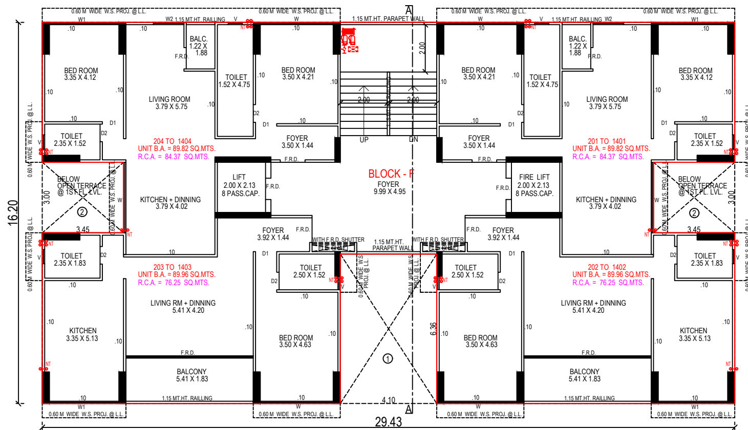
TYPICAL FLOOR PLAN (2ND. TO 14TH. FLOOR PLAN) (BLOCK - F)
