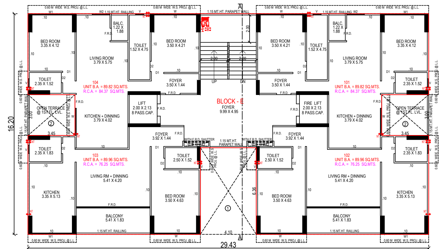
1ST. FLOOR PLAN (BLOCK - E)
