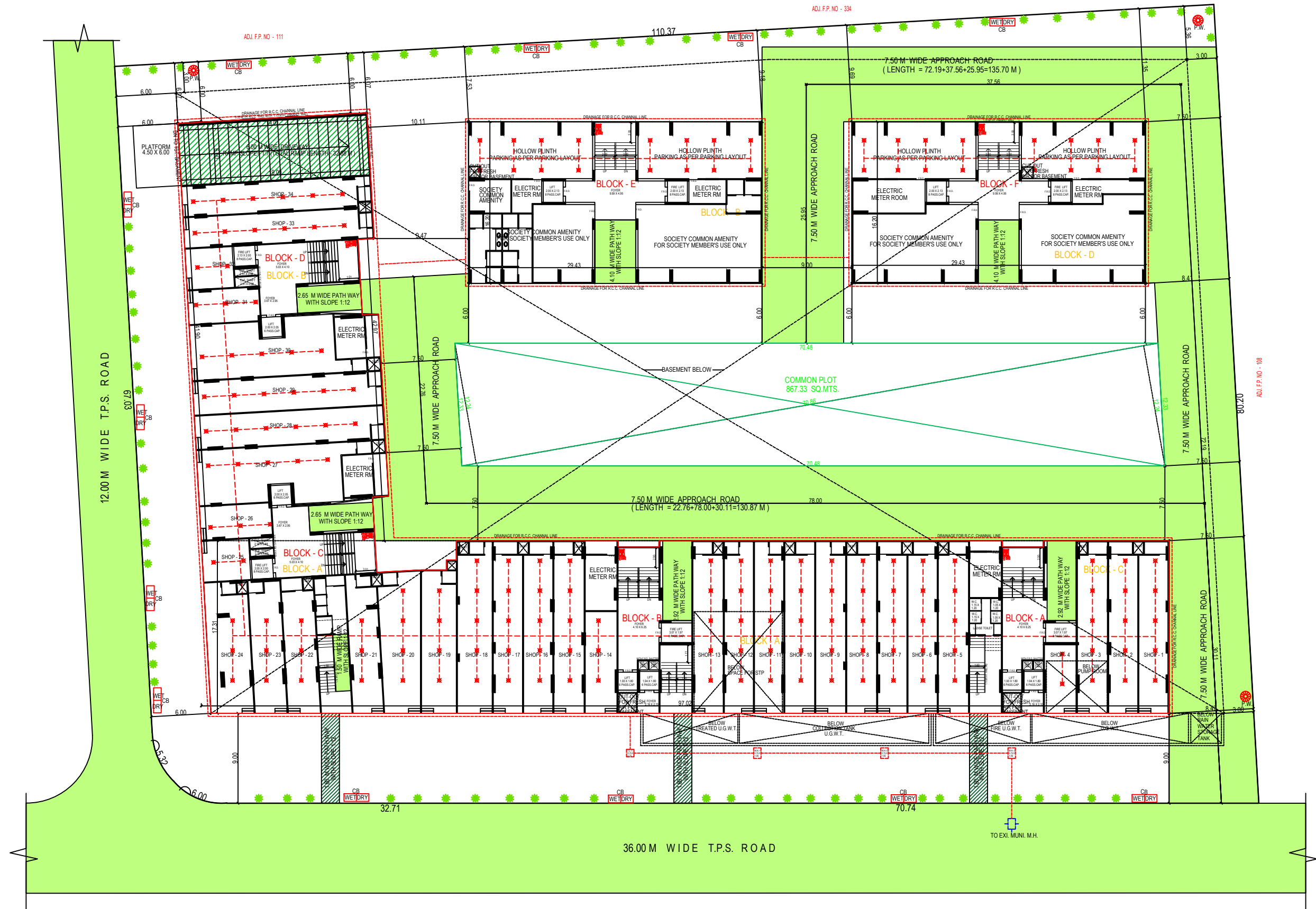
LAYOUT PLAN
