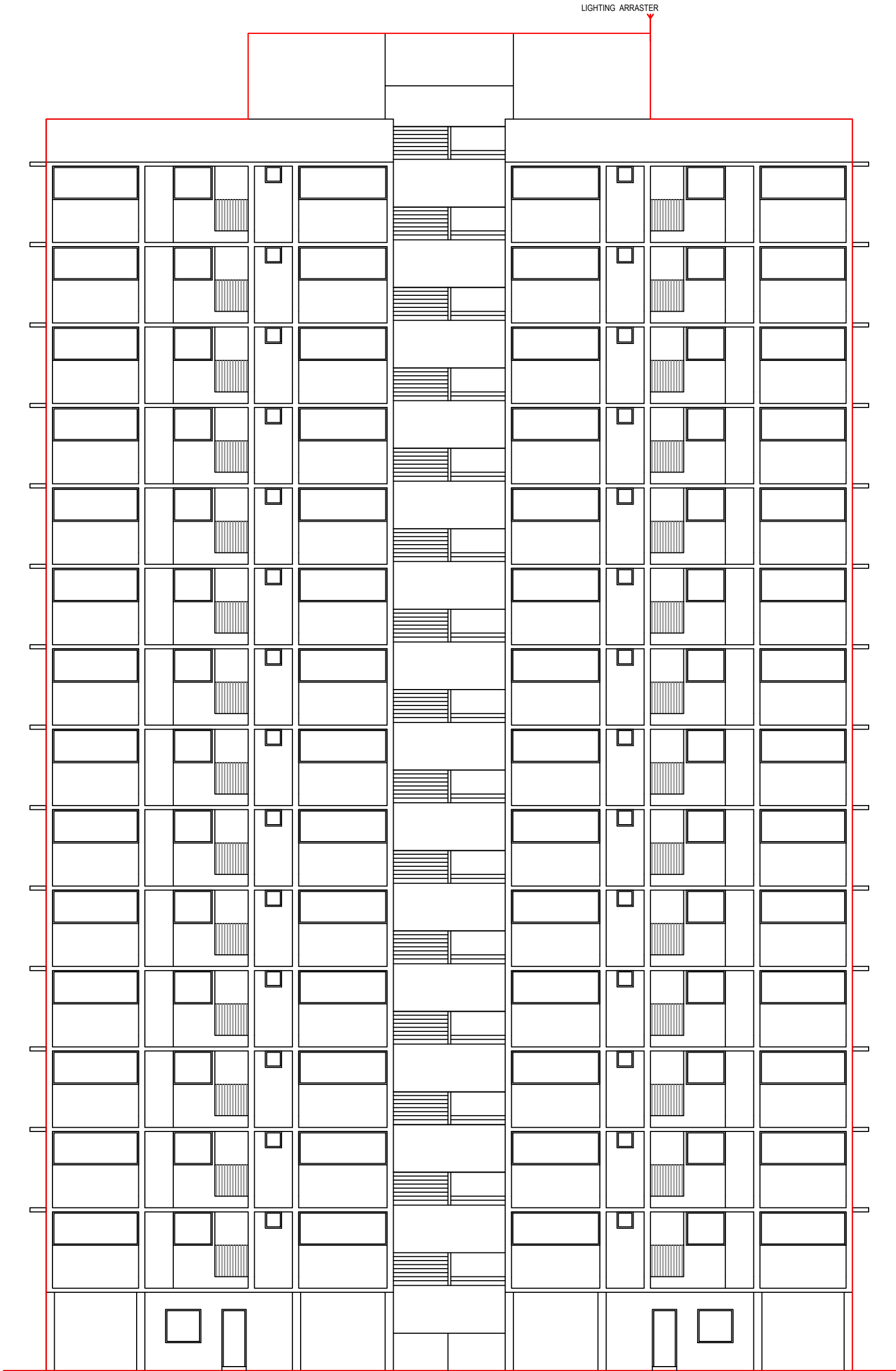
ELEVATION (BLOCK - E)
